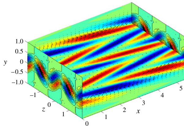
FIGURE 13. (Colour online) Velocity field of the perturbation that optimally excites the least-damped sinuous mode, which has structure very close to the EE shown in figure 12. Optimal perturbations that maximize energy amplification for shorter time periods have similar structure. A unit energy initial condition in the form of this perturbation excites the sinuous mode in energy by a factor of 1900 greater than an initial condition consisting of the sinuous mode itself. It follows that the sinuous mode amplitude, and by extension the first EE of the POD, arises from perturbations in the forced turbulence almost entirely due to non-normal growth processes.
