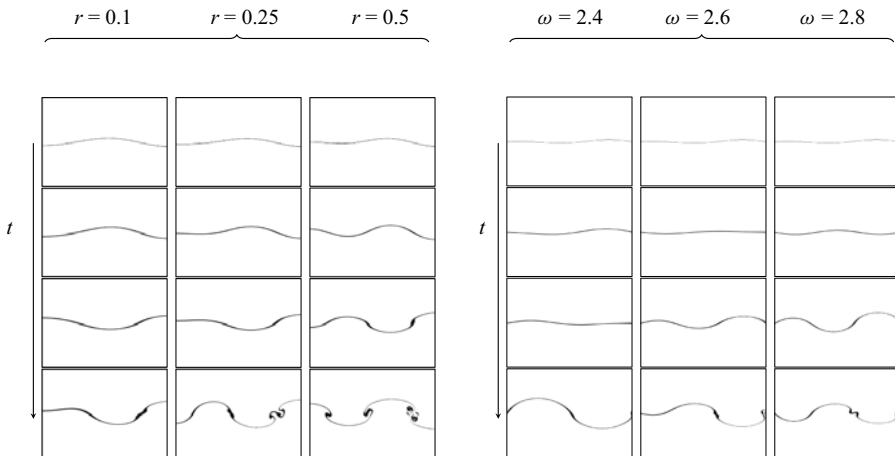
Figure 4. Mode selection in six DNS of figure 3. (a) Cases corresponding to DNSc (see table 2) with r varying and \mathcal{A} = 0.030 , \omega = 3.07 , F = 0.8 . The amplitude of the interface deformation is \epsilon = 3 cm. (b) Cases corresponding to DNSb (see table 2) with \omega varying and \mathcal{A} = 0.030 , F = 0.8 , r = 0.5 , \epsilon = 1.5 cm. We put the slices of width W of the concentration field at four instants starting from the initial interface at t = 0 and ending when the wavebreaking occurs; pure fluids remain in white, while mixed fluid with C = 0.5 \pm 0.15 is in black.
