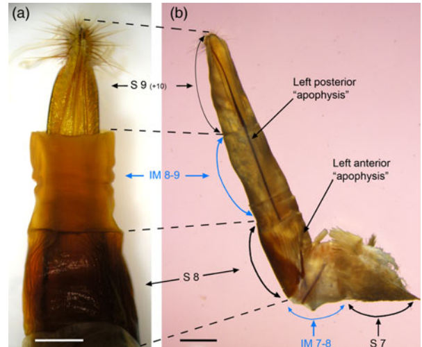
Fig. 5. P. archon ovipositor. (a) ventral view of partly retracted ovipositor (treated with potassium hydroxide 10%). (b) side view of fully everted ovipositor (segment 9 + 10, intersegment 8–9, segment 8) plus intersegment 7–8 and part of segment 7 (in ethanol 70%). Left side is dorsal; right side is ventral. Black arrows show from top to bottom the 9 (+10), 8 and 7 abdominal segments; blue arrows show the intersegmental membranes between segments 8–9 (top) and 7–8 (bottom). Left posterior and anterior 'apophysis' or apodemas are also indicated. Scale bars for a, b are 1 and 2 mm, respectively. (Photographs (a) by M.C. Santa-Cruz; (b) by V. Sarto i Monteys).
