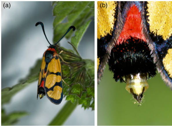
Fig. 2. Z. escalerai Poujade (Zygaenidae, Zygaeninae): (a) Calling female, (b) Closeup of ovipositor at calling, showing expanded intersegmental membrane between segments 8 and 9. (Photographs by A. Hofmann).
