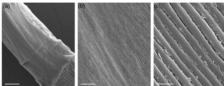
Fig. 6. SEM images of P. archon ovipositor. (a) intersegmental membrane between segments 8 and 9 showing a smooth surface ( \times 35 ). (b) closeup, 700\times showing multiple longitudinal smooth folds, allowing for extra ovipositor expansion. (c) closeup, 5000\times . Unlike sesiids, the 8–9 intersegmental membrane of P. archon ovipositor is devoid of any cuticular buds. Scale bars for a, b, c are 500, 25, and 4\ \mu\text{m} , respectively. (Photographs by V. Sarto i Monteys).
