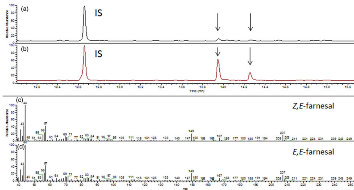
Fig. 8. GC-MS analysis (chromatogram a, b) of an extract of forewings (a) and hindwings (b) of P. archon males showing the presence of Z,E -farnesal (retention time 13.95 min) and E,E -farnesal (14.26 min) and the corresponding mass spectra (c and d, respectively). Peak at retention time 12.66 min of the chromatogram corresponds to the internal standard (IS) ( Z )-9-tetradecenol.
