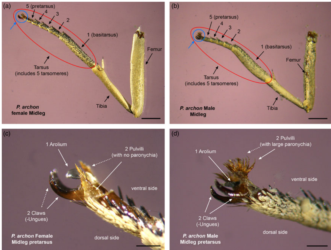
Fig. 7. Midleg of P. archon female (a) and male (b). Side view of full midleg (excluding coxa and trochanter), tibia and tarsus are seen lateroventrally. The 1st tarsomere (basitarsus) is not enlarged and appears smaller than the tibia in females (a), while in males the 1st tarsomere is notably enlarged (b). Closeup side view of pretarsal segment showing the two pulvilli with no paronychia in females (c) and forming large paronychia in males (d). Scale bars for a, b are 2 mm and for c, d 0.4 mm. (Photographs by V. Sarto i Monteys).
