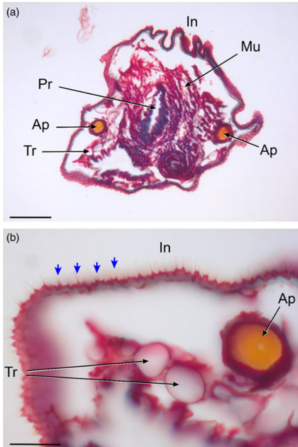
Fig. 4. Clearwing moth Synanthedon sp. ovipositor (Sesiidae): (a) 20 µm cross-section (seen with light microscope) of intersegmental membrane between abdominal segments 8 and 9 of the ovipositor (top is dorsal). In, integument; Pr, proctodeum; Mu, muscles; Ap, posterior apodema or posterior 'apophysis'; Tr, tracheae. Scale bar: 100 µm. Many cuticular buds cover the whole intersegmental cuticle, each topped with one thin and curved spinelike process, supposed to help release the pheromone. (b) closeup showing the cuticular buds (arrowheads point to some of them) of the integument. Scale bar: 30 µm. (Photographs by M.C. Santa-Cruz).
