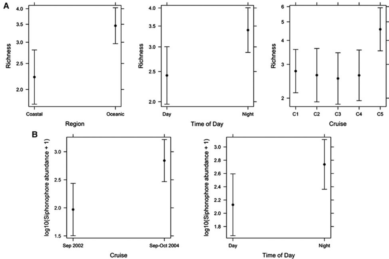
Fig. 4. Final linear models of (A) Siphonophore richness and (B) Siphonophore abundance for Sep 2002 and Sep–Oct 2004. Means ± confidence intervals are shown.
