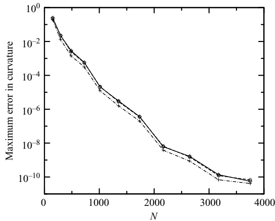
FIGURE 3. Maximum absolute error in the computed curvature versus the number of spectral points N = N_E N_B^2 for a sphere (—) and different lamellar ellipsoids: ---, a = 2 , b = 1 , c = 0.5 ; - · -, a = 4 , b = 1 , c = 0.25 (where a , b and c are the semi-axes of the ellipsoids). The exponential convergence shown in this figure was generated by employing N_E = 6 spectral elements and varying the number of basis points N_B from 5 to 25. The exact value was used to determine the numerical error.
