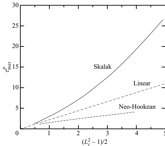
FIGURE 22. Steady-state maximum principal tension \tau_{max}^P among the spectral discretization points on the membrane as a function of strain indicator (L_c^2 - 1)/2 , where L_c is the capsule's length, for a neo-Hookean and a Skalak capsule with C = 1 in a planar extensional flow. The straight line (---) is an estimation of the initial common slope of the curves for the two capsules (based on our results for a Hookean capsule, e.g. see Barthès-Biesel et al. 2002) and denotes the linear growth of the tensions \tau_{max}^P with the strain indicator (L_c^2 - 1)/2 .
