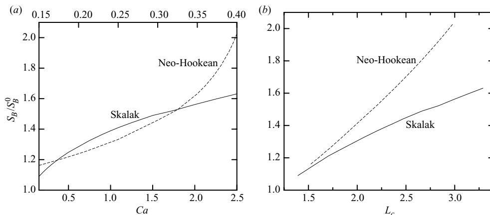
FIGURE 19. Surface area of the capsule at steady state S_B (scaled by the surface area S_B^0 of the reference spherical shape) as a function of (a) the capillary number Ca and (b) the capsule length L_c , for a neo-Hookean and a Skalak capsule with C = 1 in a planar extensional flow. Note that in (a) the neo-Hookean curve refers to the x -axis at the top of the figure.
