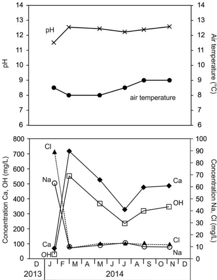
FIG. 4. Variation in chemistry of the alkaline stalactite dripwater in Peak Dale tunnel during 2014.
