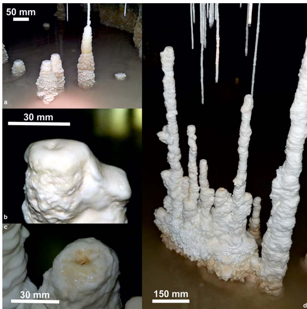
FIG. 5. Photographs of speleothems in situ . (a) A speleothem showing the frilly coating around its base, which is related to secondary flood-level growth. (b) Top of a speleothem showing side growth related to gravitational flow of unconsolidated solid calcium carbonate material and multiple drip points / excess dripping. These slippage planes can be identified in thin section. (c) When drip rates are rapid, a 'splash cup' develops. This is preserved within the structure and can be identified in the thin sections. (d) View of a group of speleothems that display examples of the morphologies highlighted in (a–c). These speleothems also demonstrate the corrugated texture along their length. The effect of migrating drips or periods when drips develop from multiple points in the tunnel roof are well evidenced in their structure.
