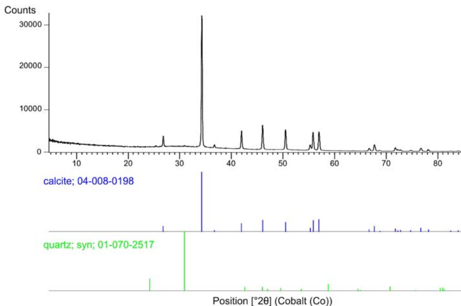
FIG. 10. XRD trace obtained from a frozen, powdered sample, washed in methanol and analysed at -20^{\circ}\text{C} in a cryogenic chamber on a PANalytical X'Pert Pro diffractometer. Several repeat analyses from different parts of the speleothem produced almost identical results. Standard 'stick' patterns for calcite ( \sim 99\% ) and trace quartz ( <1\% ) are shown.
