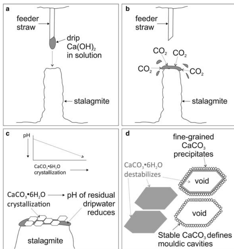
FIG. 13. Cartoon of the proposed ikaite precipitation/destabilization process. (a) High pH, \text{Ca}^{2+}\text{-OH}^- dominated dripwaters drip from the feeder straws onto the stalagmite. (b) In this air-dominated system, \text{CO}_2 is sequestered from the tunnel environment into the film of dripwater on the surface of the stalagmite. (c) The high pH stabilizes ikaite that precipitates rapidly from the dripwaters. As ikaite precipitates, this causes the pH of the dripwaters to fall. (d) The fall in pH causes the ikaite to begin to destabilize, and fine-grained calcite nucleates contemporaneously on the surface of the ikaite crystals. This replacement results in a 68% volume reduction. Finally, all ikaite destabilizes leaving fine-grained \text{CaCO}_3 that defines the mouldic cavities left by the precursor ikaite and free \text{H}_2\text{O} . This process repeats constantly with each new high-pH drip.
