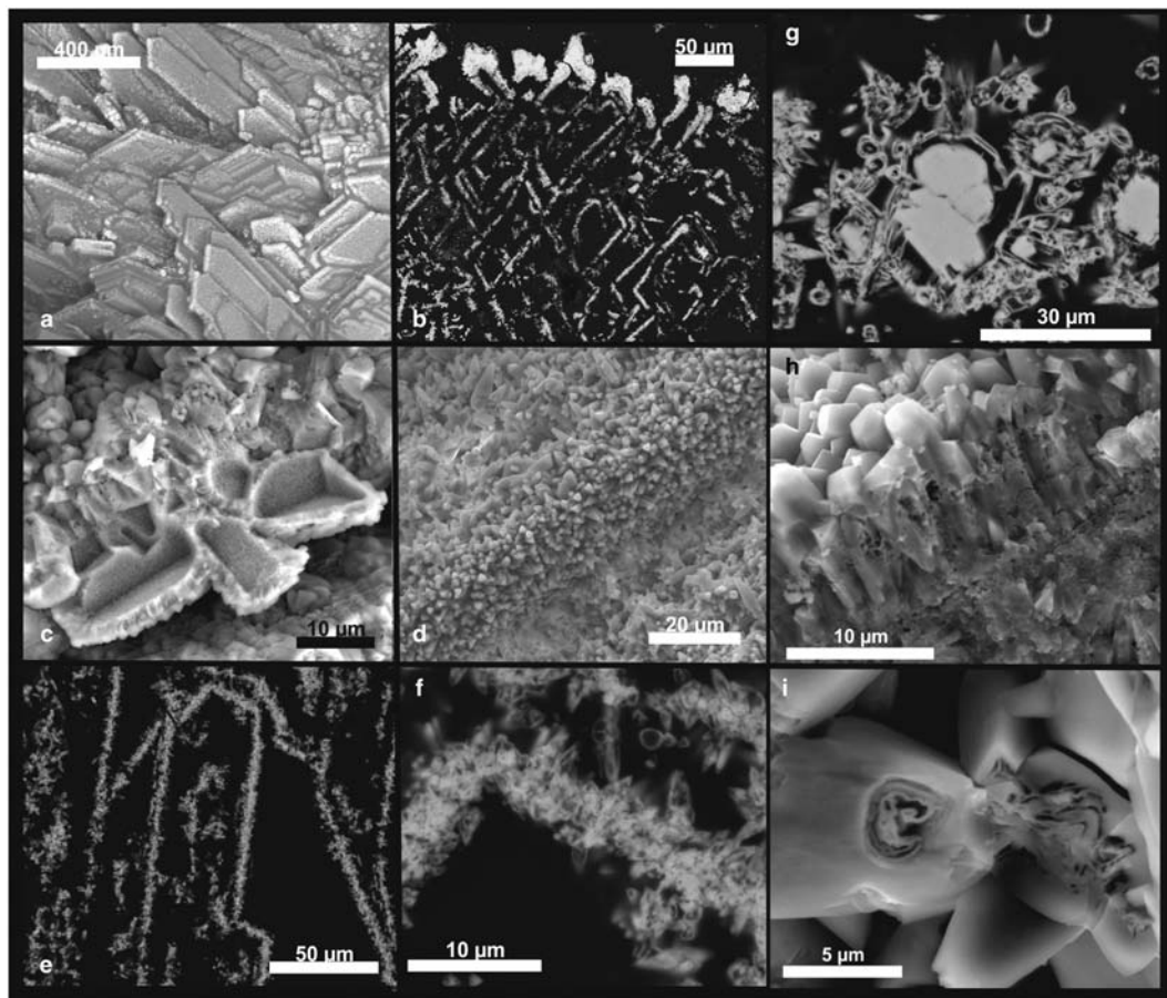
FIG. 8. ( a, b ) SE and BSEM image respectively, of pseudomorphs after ikaite. Image ( a ) shows pseudomorphs that have been coated with resin; these forms are defined by an aggregate of numerous fine-grained calcite crystals (<10 \mu\text{m} ). These small calcite crystals are visible above the level of the resin. Image ( b ) shows the hollow nature of the pseudomorphs. ( c ) SE image showing partial pseudomorph moulds. The interior is hollow, whilst the pseudomorph is defined by calcite crystals (<1 \mu\text{m} ). ( d ) SE image of the calcite aggregate defining the pseudomorph outer-coating (individual calcite crystals <10 \mu\text{m} ). ( e ) BSEM image detail of a pseudomorph outline in thin section. ( f, g ) Detail showing the skeletal nature of the individual calcite crystals that collectively define the pseudomorphs. ( h, i ) ESEM images from the cryogenic sample of these fine-grained calcite crystals. ( h ) Euhedral calcite overgrowth tips above secondary calcite. ( i ) Horizontal section through an individual calcite crystal showing fresh overgrowth around a 'cabbage leaf', skeletal interior, now entirely comprising calcite.
