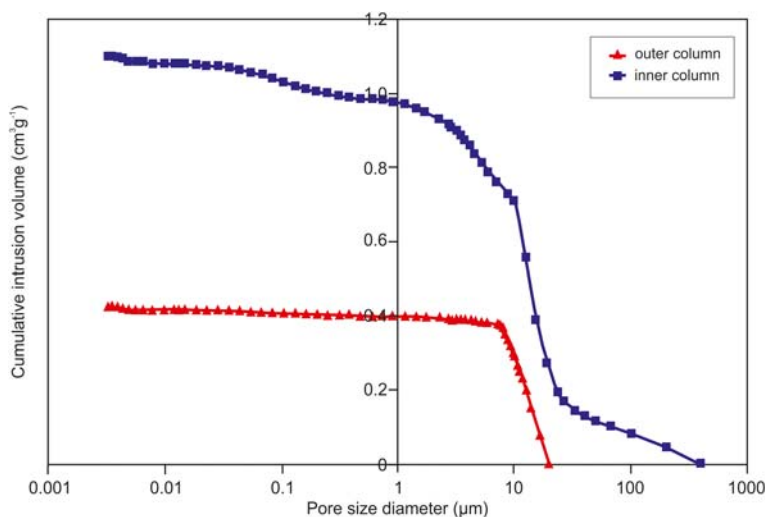
FIG. 12. MIP profiles for inner and outer columns, analysed from 0.5 to 60,000 psi.
