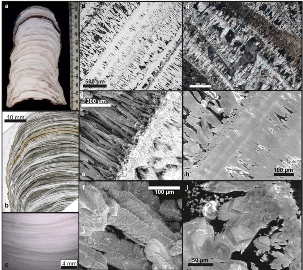
FIG. 6. Morphology of the 'small' speleothems. (a) Vertical slice through a speleothem showing a generally horizontal laminated texture. (b) Optical scanner image of part of a thin section showing pinching out of some laminae. (c) Optical microscope image of the slice showing fine laminae. (d) BSEM image showing dense laminae interspersed with porous layers of upward-growing crystals. (e) SE image showing morphology of two dense laminae interspersed with a coarser, more porous layer. (f) Detail of the crystals within the coarse layer in (e). (g) Crossed polars image showing a crystal in extinction that extends across two laminae. (h, i) CCI images showing detail of complex zoning within the crystals. Note: The observations indicate these samples comprise primary \text{CaCO}_3 (calcite dominated): these speleothems lack the evidence of pseudomorphs and an ikaite precursor identified in the subsequent, larger samples.
