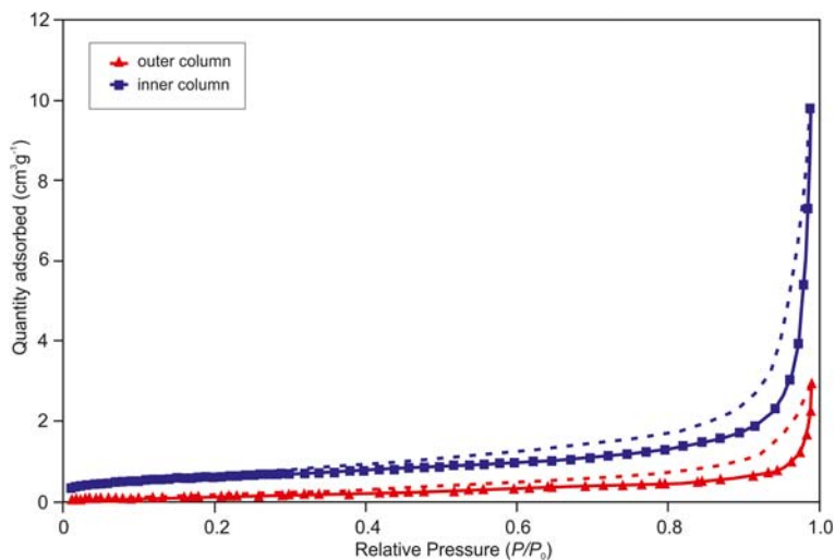
FIG. 11. Nitrogen sorption isotherms for inner and outer column samples, analysed from 0.01-0.99\ P/P_0 at -196^{\circ}\text{C} . Solid lines denote the adsorption curve, the dashed line denotes the desorption curve.
