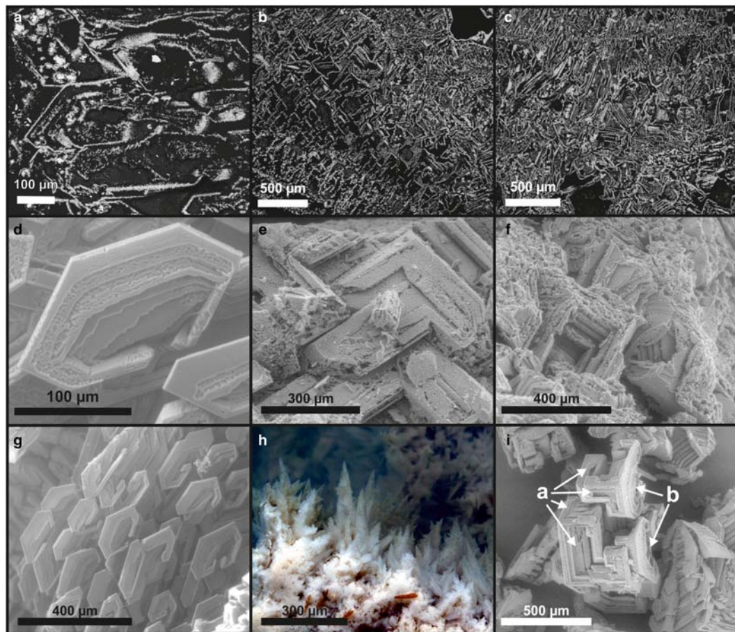
FIG. 9. Comparison of moulds from the non in situ sample ( a ); and the intact sample (thin section: b , c ); the 'cryogenic' sample ( e , f ); alongside fresh ikaite crystals (confirmed by XRD analysis: Milodowski et al. , 2013, 2014) from Harpur Hill ( d , g , h , i ). Note the close similarities between the pseudomorphed crystal form of the Peak Dale speleothem material, and actual ikaite forming at Harpur Hill (compare ( a ) to ( d ) which show a monoclinic symmetry that cannot be assigned to calcite, and ( e , f ) to ( i )). The faces labelled 'a' in ( i ) relate to those shown in ( e ) and ( f ), and the faces labelled 'b' in ( i ) relate to ( d , g ). Note that these fine-grained, complex, euhedral crystals (<200 μm: d , g ) aggregate into complex, dendritic spires. These aggregates are akin to the 'glendonite' and 'jarrowite' pseudomorphs after ikaite, more commonly preserved in the geological record.
