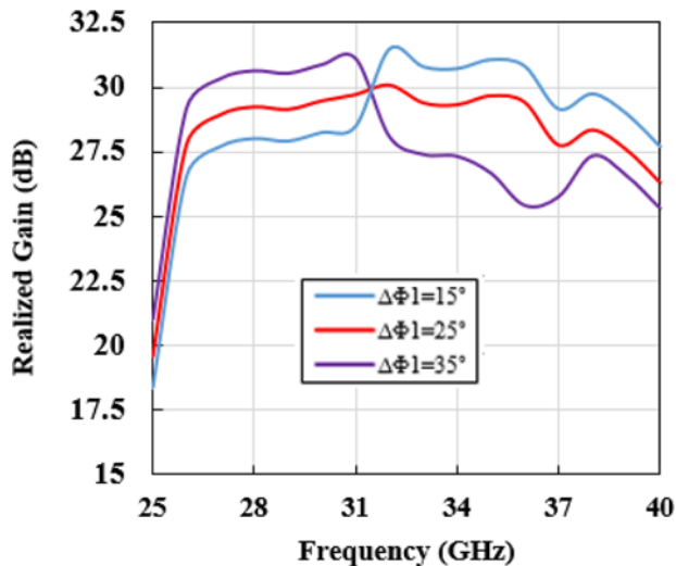
Figure 8. Simulated gain performance by adding a constant reference phase.
