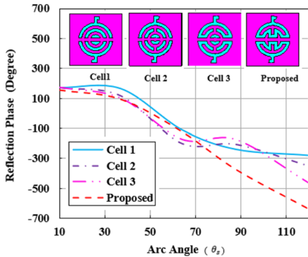
Figure 2. Reflection phase characteristics during the evolution stages.
