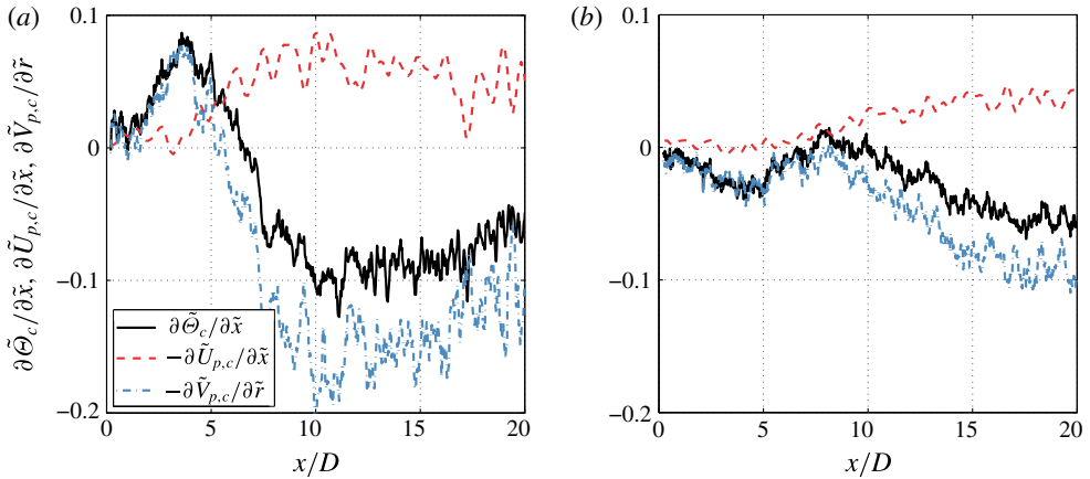
FIGURE 20. (Colour online) The normalised axial gradients of particle concentration, \partial \tilde{\Theta}_c / \partial \tilde{x} , particle axial velocity, \partial \tilde{U}_{p,c} / \partial \tilde{x} and normalised radial gradient of particle radial velocity, \partial \tilde{V}_{p,c} / \partial \tilde{r} , along the centreline for Sk_D = 1.4 (a) and Sk_D = 11.2 (b). Note that both panels use the same legend.
