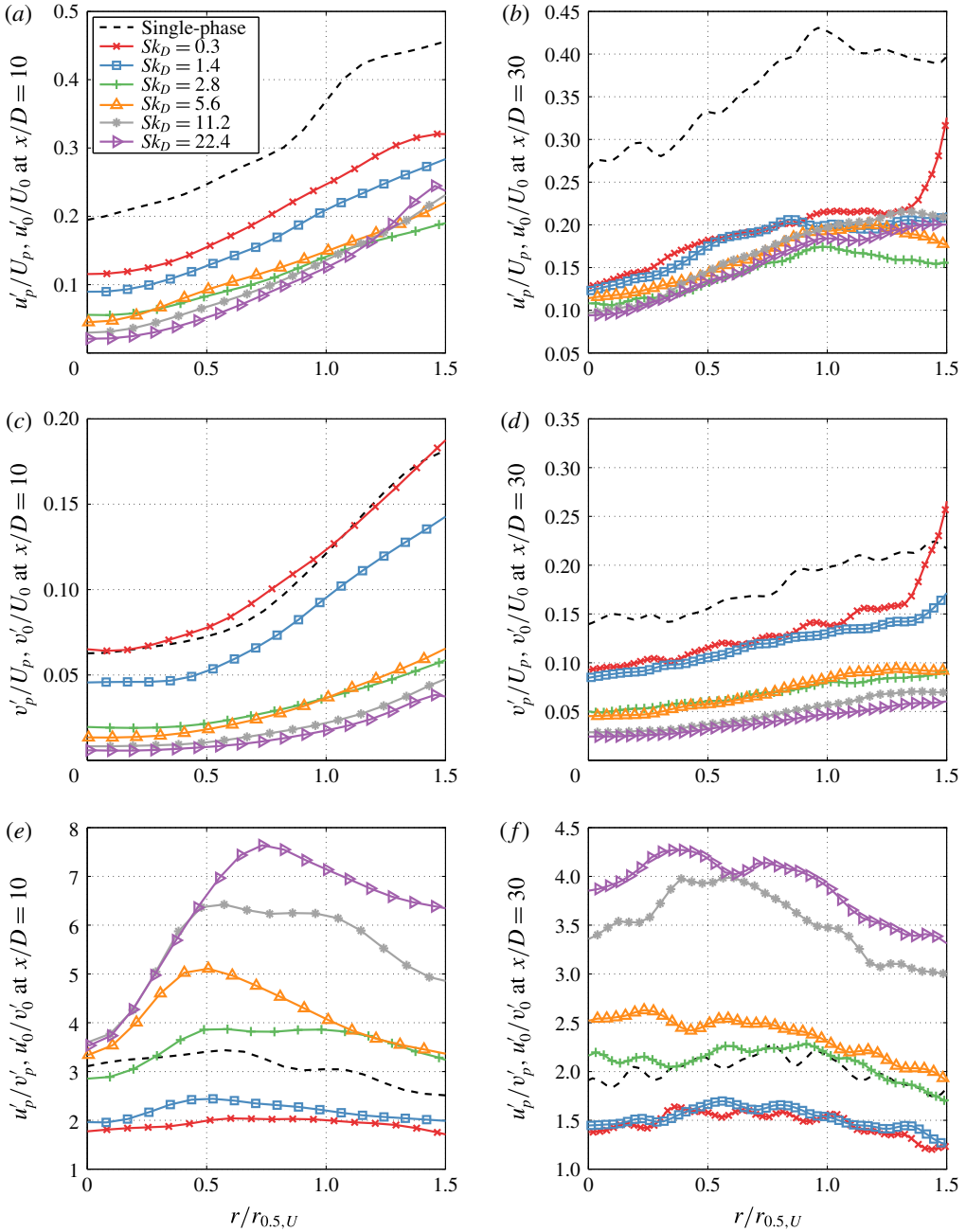
FIGURE 13. (Colour online) The axial and radial turbulence intensities, u'/U and v'/U , respectively, as well as the ratio u'/v' , as a function of normalised radial distance, r/r_{0.5,U} , for both the particle phase ( p ) and the single phase ( 0 ) at x/D=10 (a,c,e) and x/D=30 (b,d,f). Note that all panels use identical legends.
