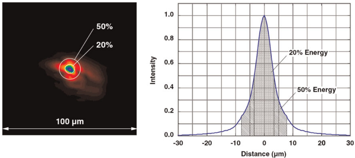
Fig. 1. (Color online) Image of focal spot in vacuo at low energy taken with a 16-bit CCD camera ( left ). Radial lineout of focal spot intensity showing 20% and 50% encircled energy boundaries ( right ). Adapted from (Patel et al. , 2005)
