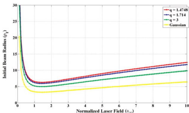
Fig. 3. (Color online) The initial (at \zeta = 0 ) dimensionless beam width ( \rho_1 ) is depicted versus the normalized laser field ( a_{00} ) for different values of the q -parameter. The relation between the ( \rho_1 ) and ( a_{00} ) is expressed by Eq. (25). The beam propagation corresponding to points ( a_{00} , \rho_1 ) which lie on these curves (critical curve) leads to relativistic guided uniform beam propagation.
