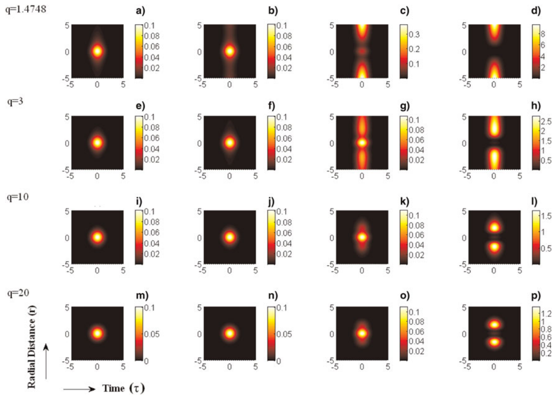
Fig. 4. (Color online) Spatial evolution of a q -Gaussian circularly polarized laser beam: the variation of the normalized intensity, as obtained from Eqs. (8) and (16), with radial distance r and time t is shown at different propagation time (equivalent to fixed propagation distance): at T_1 = 0 (first column); T_2 = 3 fs (second column); T_3 = 7 fs (third column); T_4 = 10 fs (fourth column) (corresponding to propagation distance \zeta = 0, 18 \mu\text{m}, 45 \mu\text{m} and 81 \mu\text{m} ). The radial distance ( r ) and time ( t ) are normalized by the initial beam width and initial pulse width respectively. The results are shown for different q values: q = 1.4748 (value as in Patel et al. (2005); top row); 3 (second row); 10 (third row); 20 (practically Gaussian; bottom row). The laser plasma parameters used in the computation are: a_{00} = 0.1 ( I_0 = 1.37 \times 10^{16} \text{ W/cm}^2 , \lambda = 1 \mu\text{m} ), r_0 = 30 \mu\text{m} , \tau_0 = 17 ps, n_0 = 4 \times 10^{20} \text{ cm}^{-3} and \omega = 10^{15} \text{ rad sec}^{-1} . The color bar represents the variation of the normalized intensity.
