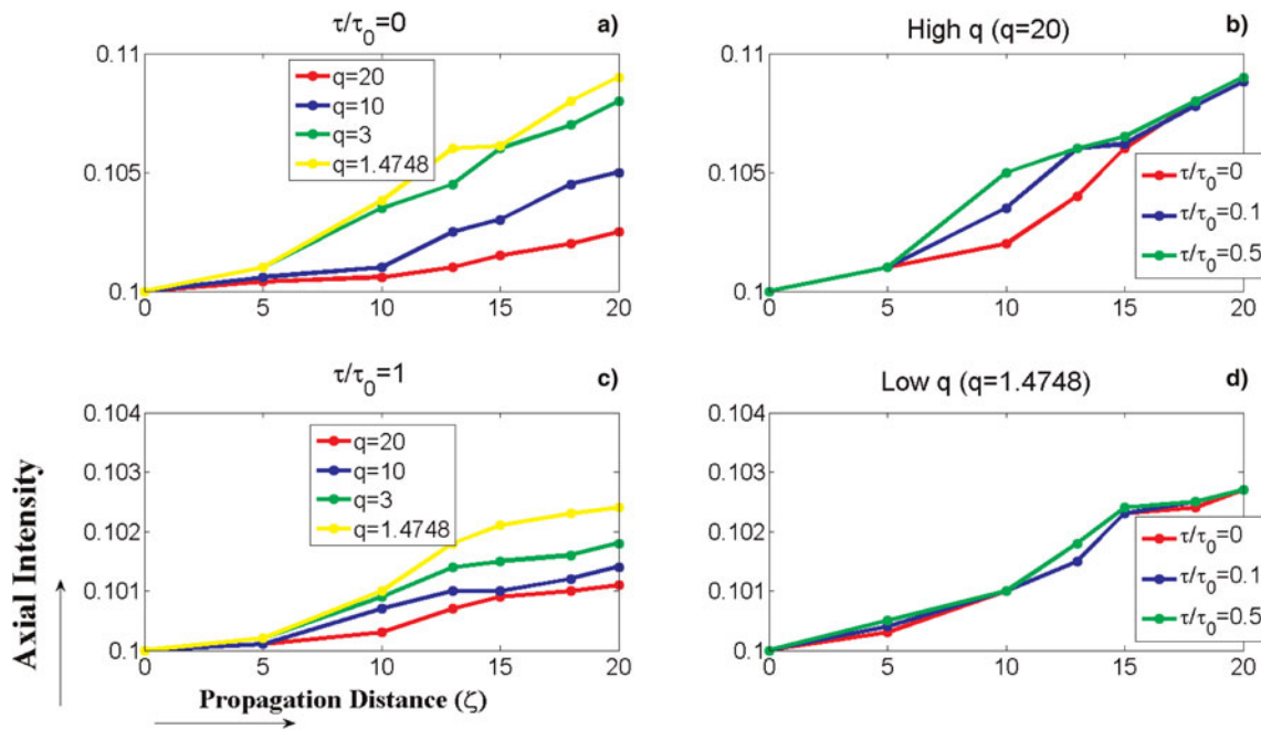
Fig. 6. (Color online) Dependence of axial intensity a^2(\rho = 0, \zeta, \tau) on the propagation distance ( \zeta ). Panels (a) and (c) show the variation of the axial intensity with \zeta for different values of the non-Gaussian parameter ( q ) at \tau/\tau_0 = 0 and \tau/\tau_0 = 1 . Panels (b) and (d) show the variation in the axial intensity along \zeta at various values of time, for high and low values of the non-Gaussian parameter q . The laser-plasma parameters used for the numerical computation are the same as in Figure 4.
