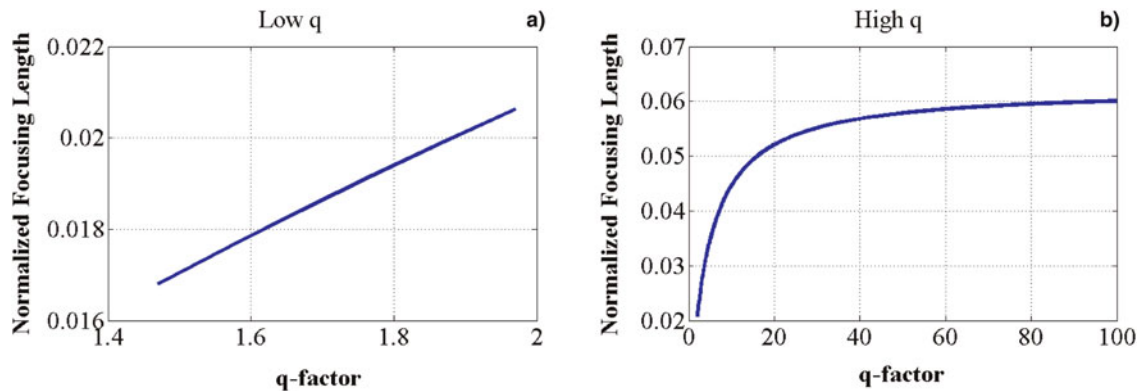
Fig. 5. (Color online) The dependence of the normalized focusing length on the non-Gaussianity parameter q is depicted. The focusing length ( \rho_1 \omega / \omega_{p0} \sqrt{2} ) is normalized by the diffraction length ( kr_0^2 ). The laser-plasma parameters used for the numerical computation are the same as in Figure 4.
