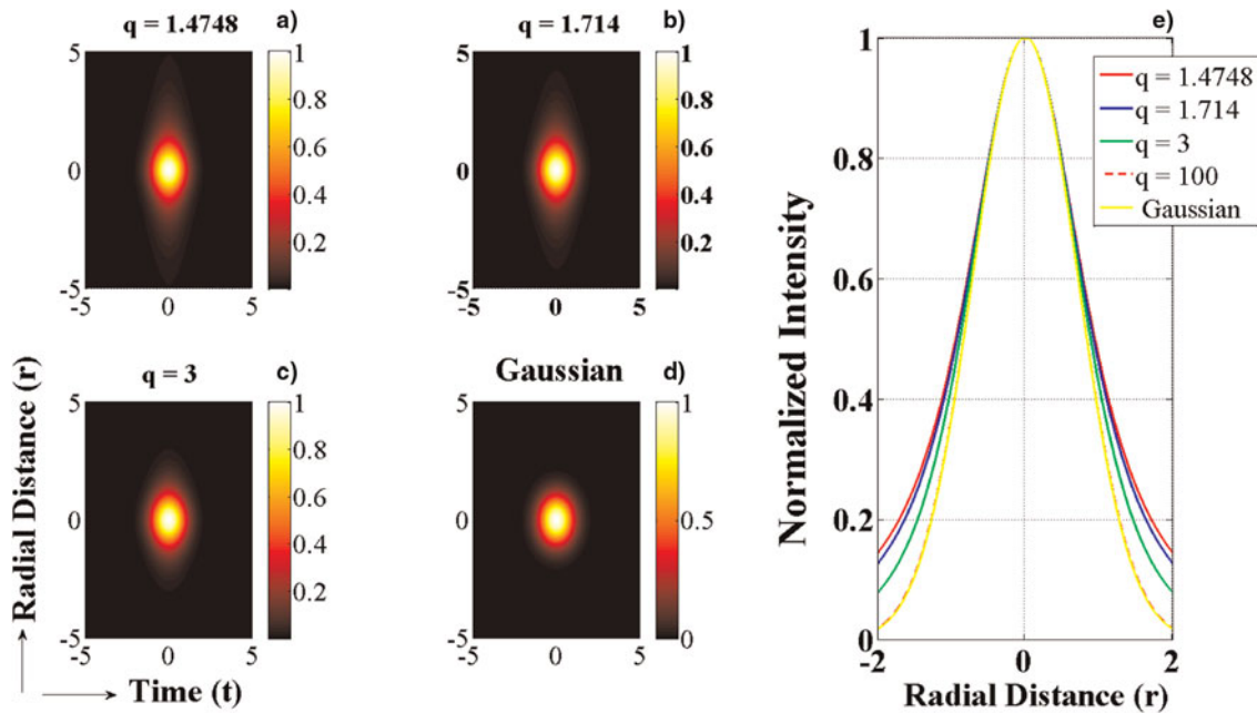
Fig. 2. (Color online) Initial intensity profile of the q -Gaussian laser pulse for q = 1.4748, 1.714, 3, and \infty ; from (Eqs. 8 and 7). The radial distance ( r ) and time ( t ) are normalized by the initial beam width and initial pulse width respectively. Panels (a)–(d) show the normalized 3D intensity initial snapshots of a q -Gaussian laser pulse whose spatial beam radius ( r_0 ) is 30 \mu\text{m} and temporal pulse duration ( \tau_0 ) is 17 ps, respectively. Figure 2e shows the spatial intensity profiles of q -Gaussian beam. The color bar represents the variation of the initial intensity. The long tail associated with small q is clearly visible.
