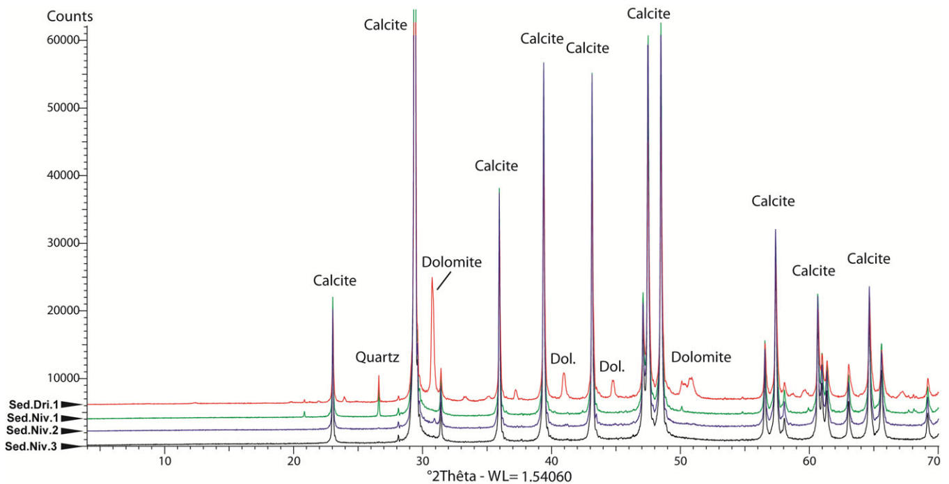
Fig. 4. (Colour online) X-ray diffractograms of the lithographic limestone from Drigas and Niveliers. Dol. – dolomite; WL – wavelength.
