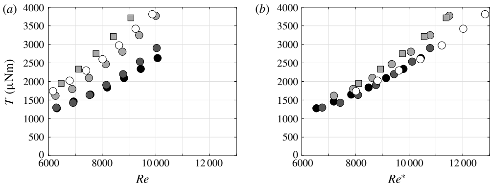
FIGURE 3. Water-filled groove cylinder torque with Reynolds number based on (a) gap height d and (b) effective gap height d_{eff} . Groove sizes are w = 100 \mu\text{m} (black), 200 \mu\text{m} (dark grey), 400 \mu\text{m} (light grey) and 800 \mu\text{m} (white); fluid area fractions a = 0.5 (circles) and 0.85 (squares).
