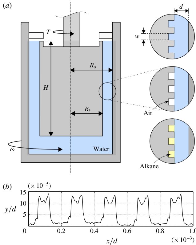
FIGURE 2. (Colour online) (a) Experimental set-up of the Taylor–Couette facility. Longitudinal grooves are tested with water (baseline), air (superhydrophobic) or alkane oils (liquid-infused). (b) Sample confocal microscope measurements of the smallest groove size, w = 100 \mu\text{m} .
