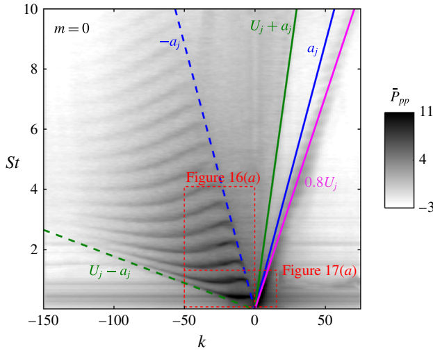
FIGURE 11. (Colour online) Frequency–wavenumber diagram ( \square \blacksquare , \bar{P}_{pp}(0 \leq x \leq 5, r_0) ) of the LES data in the potential core region for m=0 and r_0=0.1 . Lines of constant propagation velocity c_p = \omega/k = c_g = \partial\omega/\partial k and their corresponding values are shown in colour. c_p = 0.8U_j corresponds to the propagation speed of K–H instabilities.
