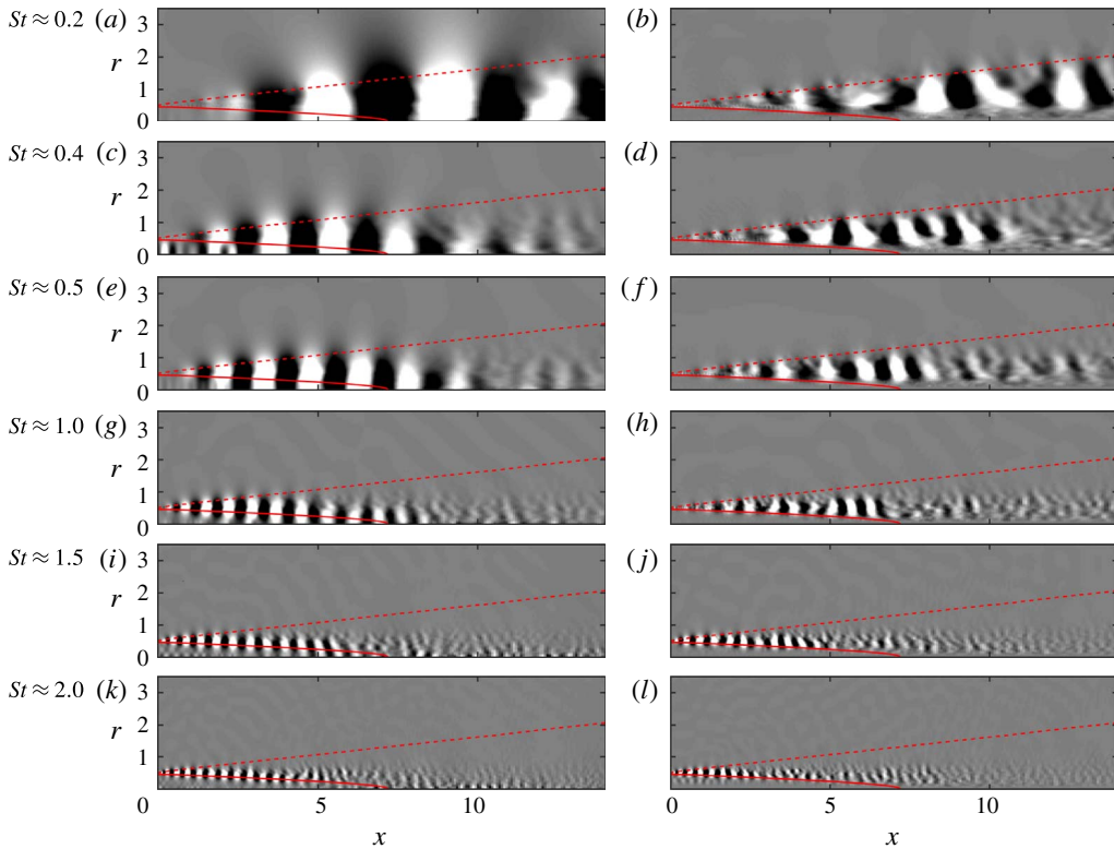
FIGURE 3. (Colour online) Spectral estimation of pressure POD modes ( \square , -0.25 \leq \Psi_p / \|\Psi_p\|_\infty \leq 0.25 ) for different Strouhal numbers: (a,c,e,g,i,k) m=0 ; (b,d,f,h,j,l) m=4 .
