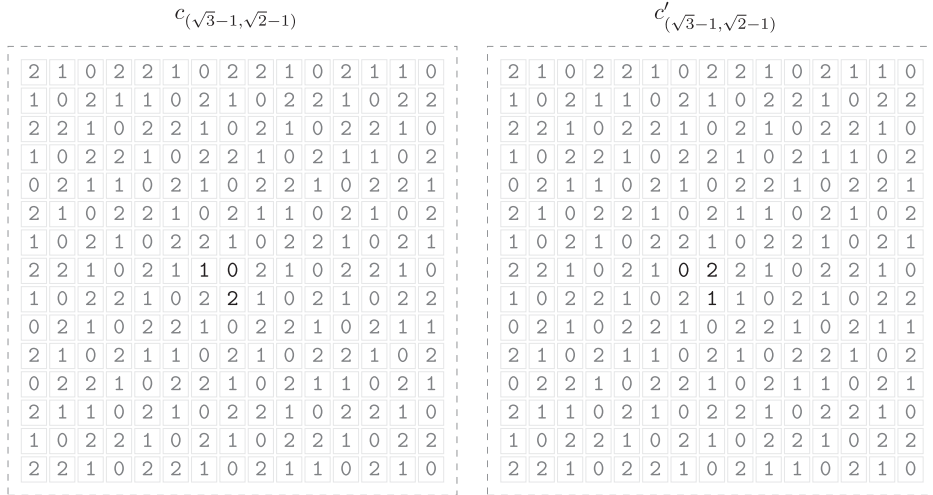
FIGURE 9. Two-dimensional configurations c_\alpha and c'_\alpha when \alpha = (\sqrt{3} - 1, \sqrt{2} - 1) are shown on the support [-7, 7] \times [-7, 7] . The two configurations are equal except on the difference set F = \{(0, 0), (-1, 0), (0, -1)\} shown in darker hue.
