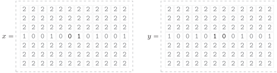
FIGURE 7. An indistinguishable, recurrent, but not uniformly recurrent asymptotic pair (x, y) given by the two characteristic Fibonacci words (\alpha = (\sqrt{5} - 1)/2) in the central row.
