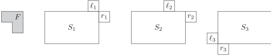
FIGURE 8. (S_1, \ell_1, r_1) is evil, as both \ell_1 and r_1 can simultaneously overlap F without S_1 doing so. Notice that (S_2, \ell_2, r_2) is not evil since \ell_2 - r_2 \notin F - F . (S_3, \ell_3, r_3) is also not evil since the unique t \in \mathbb{Z}^2 with t + \{\ell_3, r_3\} \subset F is such that (t + S_3) \cap F \neq \emptyset .
