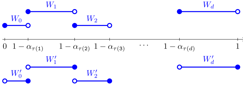
FIGURE 10. Define \alpha_0 = 1 and \alpha_{d+1} = 0 , and let \tau be the permutation of \{1, \dots, d\} \cup \{0, d + 1\} which fixes \{0, d + 1\} and such that 0 < \alpha_{\tau(d)} < \dots < \alpha_{\tau(1)} < 1 . The intervals W_i = [1 - \alpha_{\tau(i)}, 1 - \alpha_{\tau(i+1)}) form a partition of the circle \mathbb{R}/\mathbb{Z} and similarly for the intervals W'_i = (1 - \alpha_{\tau(i)}, 1 - \alpha_{\tau(i+1)}) .
