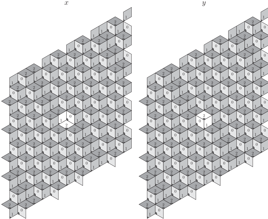
FIGURE 3. Configurations x and y from Figure 1 are encoding a tiling of the plane [5] by three types of pointed rhombus drawn using Jolivet’s notation [23, p. 112]. The tilings shown above correspond to the projection of the surface of a discrete plane of normal vector (1 - \alpha_1, \alpha_1 - \alpha_2, \alpha_2) \approx (0.293, 0.348, 0.359) , with \alpha = (\alpha_1, \alpha_2) = (\sqrt{2}/2, \sqrt{19} - 4) , in three-dimensional space, and their difference can be interpreted as the flip of a unit cube shown in white.
