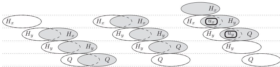
FIGURE 13. The pattern \pi(x)|_{S \cup (S-t-e_1) \cup (S-2t-2e_1)} , shown in gray, appears in \pi(y) intersecting the difference set F \setminus \{-e_1\} in one of three ways. To lighten the figure, we omit the shifts \sigma^{e_1+t} in the ellipses. In the first case, the non-trivial overlap of H_y with itself is impossible, which implies H_x = H_y , which is a contradiction. In the second case, the non-trivial overlap of H_y with itself is impossible, which implies that H_y = Q . In the third case, the proof uses the existence of patterns u_x and u_y .
