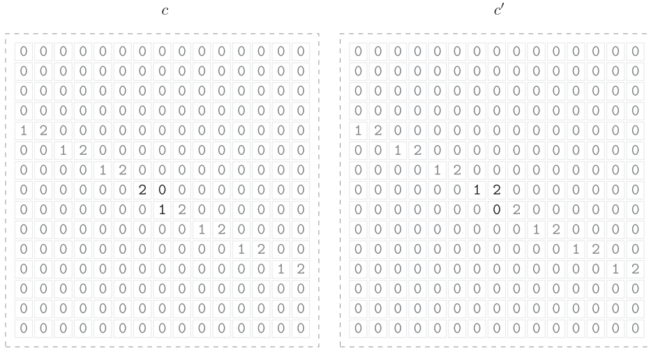
FIGURE 4. An indistinguishable asymptotic pair (c, c') which satisfies the flip condition obtained by taking the limit of the Sturmian configurations given by \alpha_n = (1/n(\sqrt{2} - 1), 1/n(\sqrt{3} - 1)) .
