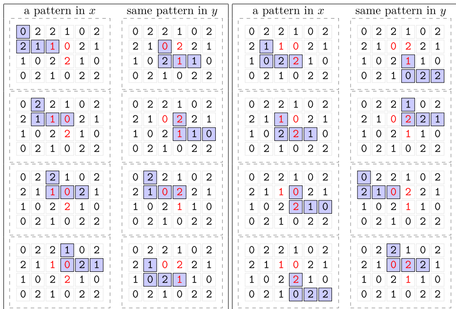
FIGURE 2. The eight patterns of shape \{0, e_1, 2e_1, e_2\} appearing in the configurations x and y . All of them appear intersecting the difference set in x and y .
