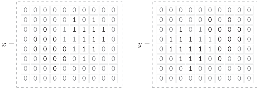
FIGURE 6. A non-trivial indistinguishable asymptotic pair for \Sigma = \{0, 1\} and d = 2 , where y = \sigma^{(3,1)}(x) . The difference set is highlighted in darker hue and the portions of the configurations which are not shown consist only of the symbol 0.
