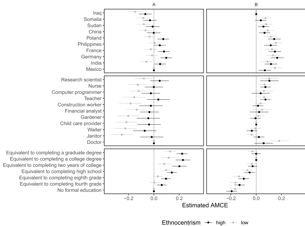
Figure 4. Comparison of AMCEs for low- and high-ethnocentrism respondents using two alternative reference category choices for three features from Hainmueller et al. 's (2014) immigration experiment.
