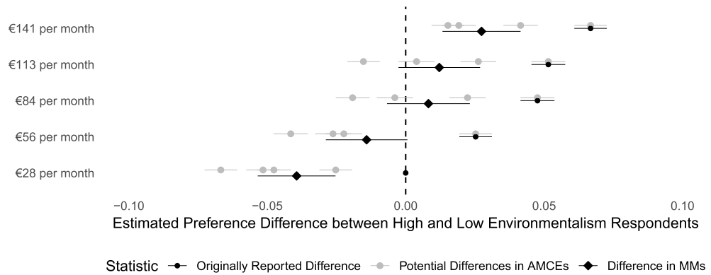
Figure 3. True difference in favorability and implied preference differences between high- and low-environmentalism respondents for “monthly cost” feature from the Bechtel and Scheve (2013) climate agreement experiment for each possible reference category.
