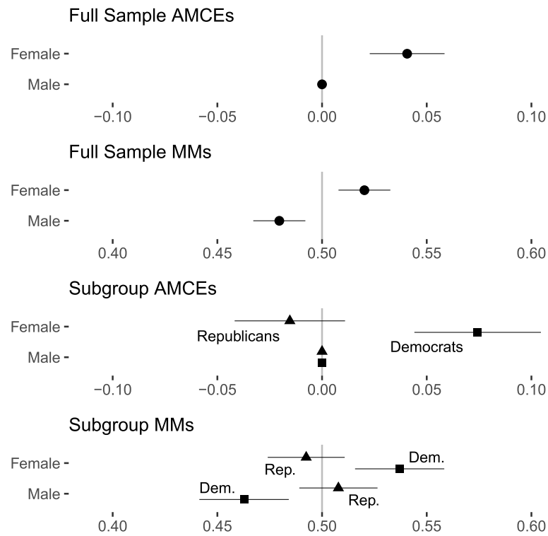
Figure 2. Replication of results for “candidate sex” feature from the Teele, Kalla, and Rosenbluth (2018) candidate experiment using full sample AMCEs and marginal means (MMs) and subgroup AMCEs and MMs for Democrats and Republicans.
