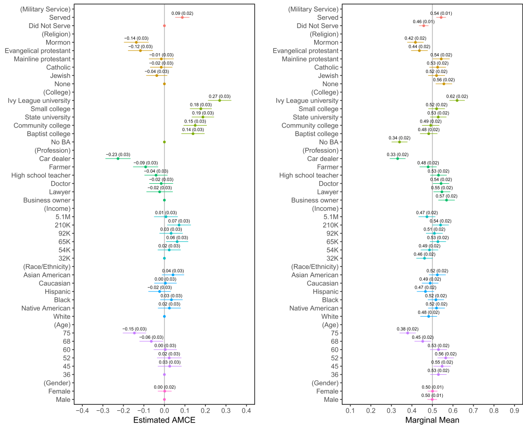
Figure 1. Replication of the Hainmueller, Hopkins, and Yamamoto (2014) candidate experiment using AMCEs and MMs.
