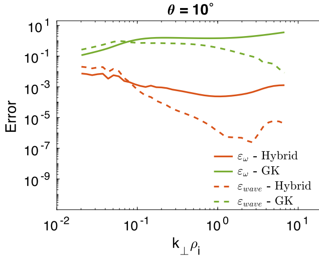
FIGURE 8. Errors for Alfvén/ion-cyclotron wave with \theta = 10^\circ , as functions of k_{\perp}\rho_i . Red and green curves are for hybrid and gyrokinetic models, respectively. Solid lines denote \epsilon_{\omega} and dashed lines denote \epsilon_{wave} .
