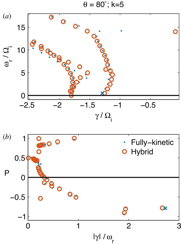
FIGURE 2. Normal modes for \theta = 80^\circ and k\rho_i = 5 for fully kinetic (blue dots) and hybrid (red circles) models. (a) Solutions in the complex plane ( \gamma, \omega_r ). (b) Solutions plotted as functions of |\gamma|/\omega_r (horizontal axis) and polarization P (vertical axis). In both panels the kinetic Alfvén wave is denoted with a blue cross.
