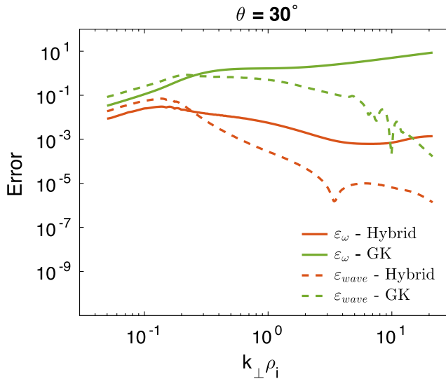
FIGURE 9. Errors for Alfvén/ion-cyclotron wave with \theta = 30^\circ , as functions of k_{\perp}\rho_i . Red and green curves are for hybrid and gyrokinetic models, respectively. Solid lines denote \epsilon_{\omega} and dashed lines denote \epsilon_{wave} .
