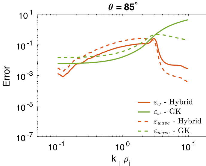
FIGURE 13. Errors for Alfvén/ion-cyclotron wave with \theta = 85^\circ , as functions of k_{\perp}\rho_i . Red and green curves are for hybrid and gyrokinetic models, respectively. Solid lines denote \epsilon_{\omega} and dashed lines denote \epsilon_{wave} .
