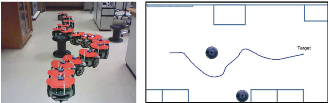
Fig. 53. Trajectory to the target, constant tangential velocity.
