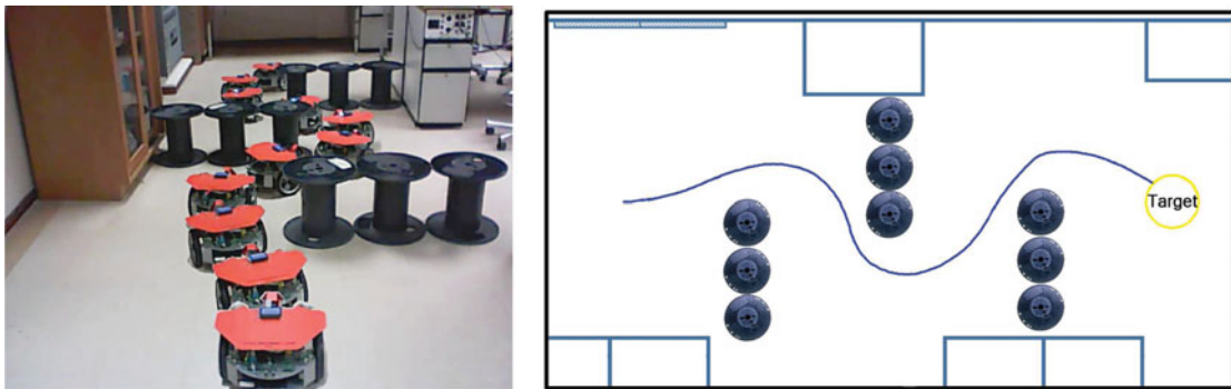
Fig. 41. Trajectory to the target, obstacle course and model-based.
