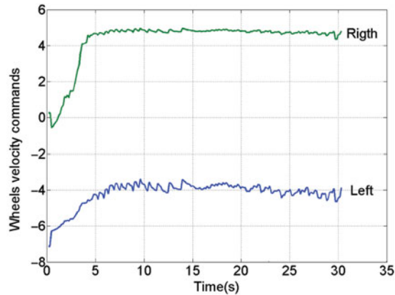
Fig. 34. Actuation signals corresponding to the trajectory in Fig. 30.
