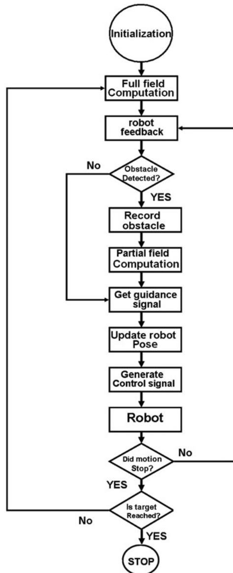
Fig. 22. The ultrasonic navigation control structure.
