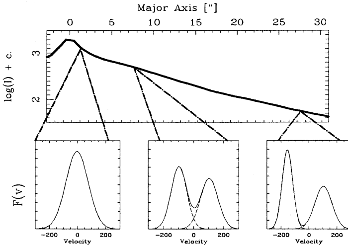
Figure 1: Major Axis Kinematics of NGC 4550
