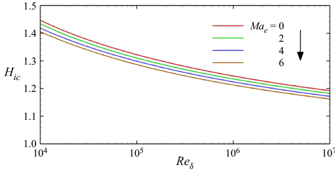
Figure 13. Dependence of incompressible shape factor H_{ic} on Mach number and Reynolds number under an adiabatic wall condition.
