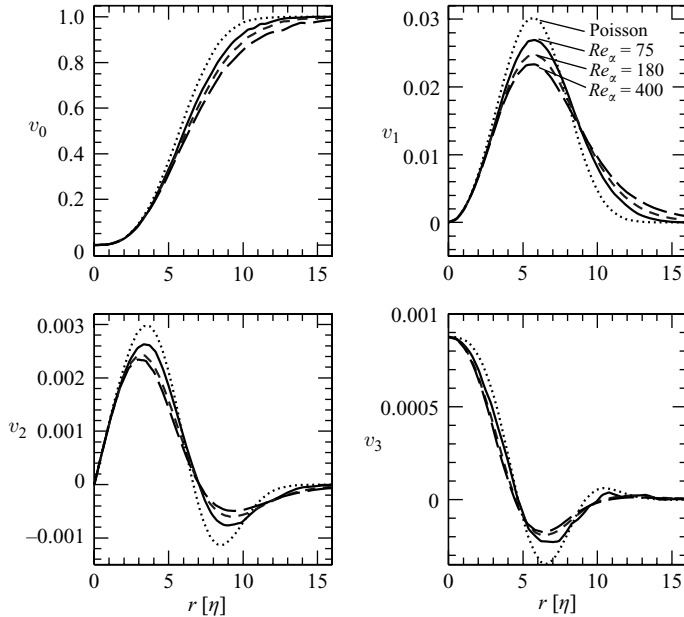
FIGURE 9. Volume densities of the Minkowski functionals v_\mu(r) , \mu=0, 1, 2, 3 for particles with \beta=0 and St=0.6 in simulations with different Reynolds numbers: Re_\lambda=75 (solid), Re_\lambda=180 (short dashed), Re_\lambda=400 (long dashed). Poisson distribution behaviour is reported for reference (dotted). All point sets have been subsampled to the same number density.
