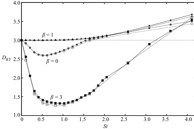
FIGURE 3. The Kaplan–Yorke dimension D_{KY} vs. St for three \beta values: \beta=0 ( \circ ), 1 ( \Delta ), 3 ( \square ). Results at two different Re_\lambda are reported: Re_\lambda=75 (filled symbols), Re_\lambda=180 (open symbols).
