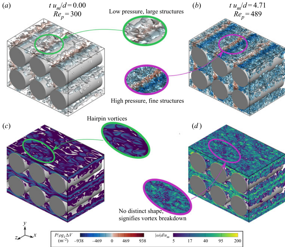
Figure 13. Transition in the three-dimensional flow features before symmetry breaking due to increase in g_i . Three-dimensional turbulent structures coloured by pressure are visualized in the sub-volume ( 3s, 2s, 2s ) of the REV-T using iso-surfaces of Q(d/\langle u_1 \rangle^i)^2 = 50 . Turbulent structures are identified by the vorticity magnitude distribution shown on the boundary of the REV-T. Vorticity contours below a magnitude of 5 are not displayed.
