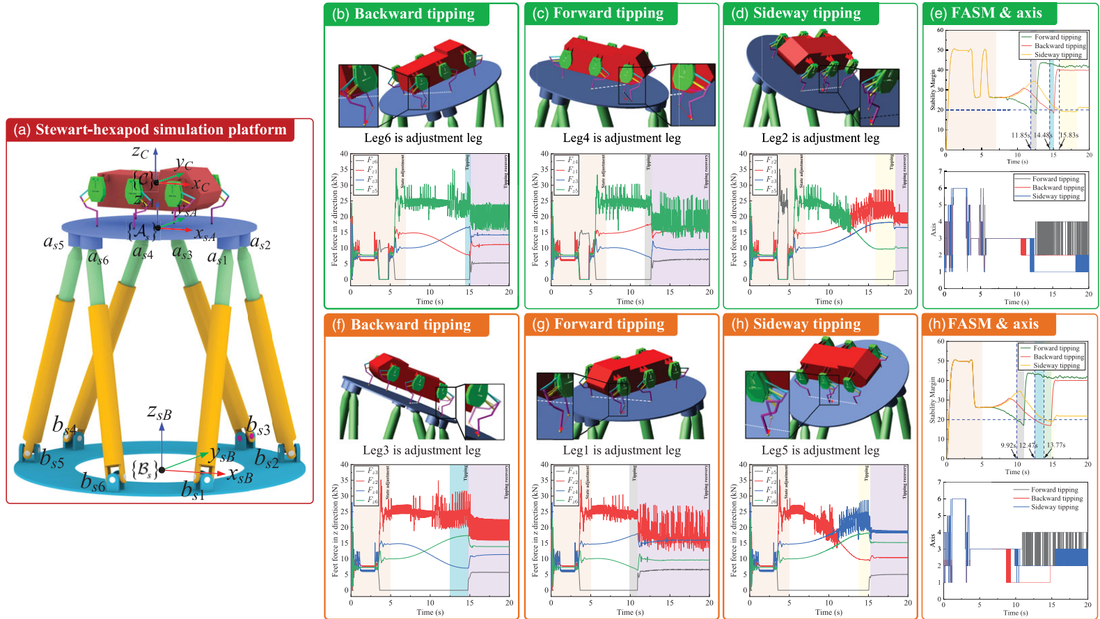
Figure 6. Stewart-hexapod platform and tipping recovery simulation. (a) represents the combined Stewart-hexapod robot simulation platform, consisting of a 6-UPS Stewart parallel mechanism and the heavy-duty hexapod robot. (b)–(d) illustrate the robot’s backward, forward, and sideline tipping recovery with legs 1, 3, and 5 in stance and the corresponding foot force in z direction. The top chart of (e) depicts the stability margin, while the bottom chart depicts the tipping rotation axis. Similarly, (f)–(h) demonstrate the robot’s backward, forward, and sideline tipping recovery with legs 2, 4, and 6 stance and the corresponding foot force in z direction. The top chart (i) showcases the stability margin variation curve, and the bottom illustrates the corresponding tipping rotation axis.
