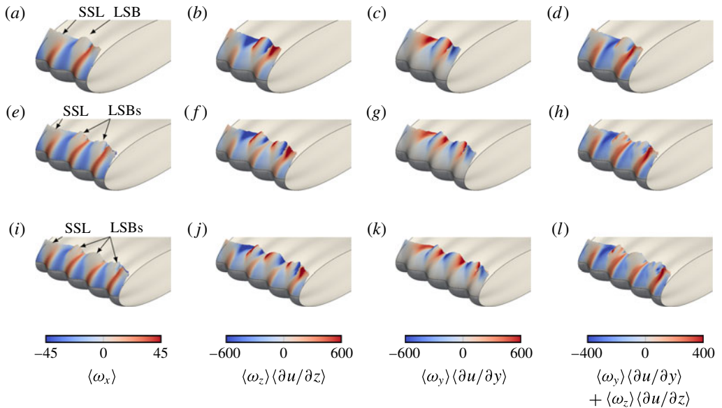
FIGURE 14. (Colour online) Iso-surfaces of time-averaged vorticity magnitude \langle |\boldsymbol{\omega}| \rangle = 45 coloured by (a,e,i) streamwise vorticity; (b,f,j) streamwise turning of spanwise vorticity; (c,g,k) streamwise turning of vertical vorticity; and, (d,h,l) the sum of the turning components. For three different WLEs: (a–d) WLE-2; (e–h) WLE-3; and, (i–l) WLE-4 cases. SSL represents the fully separated shear layer from the isolated trough without an LSB.
