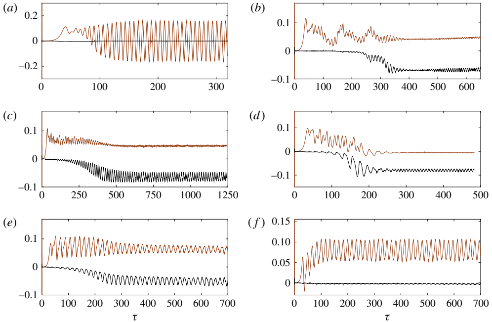
FIGURE 10. (Colour online) Time history of the force coefficients in the y and z directions ( C_{ly} and C_{lz} respectively); C_{ly} is shown with the orange colour (light) curves while C_{lz} is shown with the black colour (dark) curves; \tau = tU/D is the non-dimensional time: (a) case A at U^* = 7 , (b) case B at U^* = 10.5 , (c) case C at U^* = 15 , (d) case D at U^* = 20 , (e) case E at U^* = 28 and (f) case F at U^* = 75 . See figure 4 for the locations of the points A–F on the sphere response curve.
