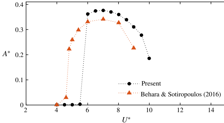
FIGURE 6. (Colour online) Comparison of VIV response for a sphere free to move only in the transverse direction ( y only), ●, and free to move in all three spatial directions by Behara & Sotiropoulos (2016) when the sphere is moving in a linear path in the transverse plane ( xz plane), ▲ (orange), at a Reynolds number of Re = 300 and a mass ratio of m^* = 3.8197 ( m_r = 2 ).
