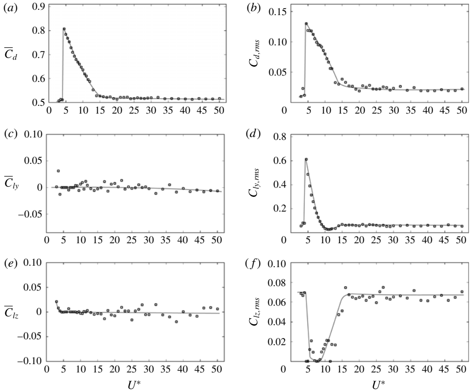
FIGURE 25. Variation of the time-mean force coefficients (a,c,e) and the r.m.s. of the fluctuation components of the force coefficients (b,d,f) in the x , y and z directions with the reduced velocity, U^* , at Re = 800 . The drag force is measured in the x direction and the lift forces are measured in the y and z directions.
