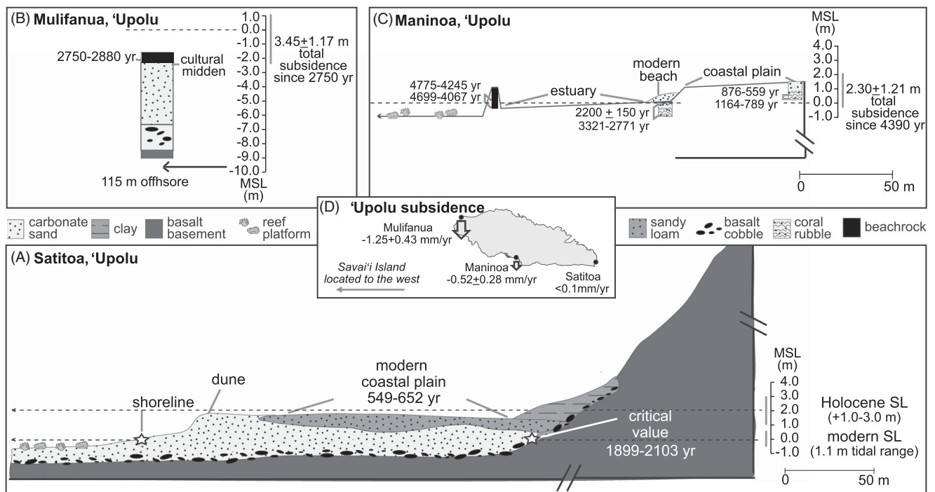
Figure 2. 'Upolu Island coastal stratigraphy interpreted at Mulifanua (after Dickinson and Green, 1998), Maninoa (after Goodwin and Grossman, 2003), and Satitooa (this study) as a function of Holocene sea-level change and local tectonics. All ages are reported as calendar years before present (cal yr BP). (A) We define the value below which sea level must fall for a carbonate coast to prograde seaward as the critical value of sea level. Following the 1–3 m modeled mid-Holocene high stand, coastal progradation at Satitooa was initiated as sea level fell beneath a critical value of 0.3–1.0 m (approximately 1899–2103 cal yr BP), and the coastal zone switched from a transgressive to a regressive environment. (B) The general stratigraphy at Mulifanua reveals paleobeachrock that formed as beach sands were cemented within the intertidal zone approximately 2750–2880 cal yr BP. The entire unit is now a submerged feature approximately 115 m offshore because of local subsidence ( 3.45 \pm 1.17 m total subsidence). (C) Offshore paleobeachrock formed at Maninoa prior to 4000 cal yr BP and subsided ( 2.30 \pm 1.21 m) to its current position within the modern intertidal zone. The coast prograded 50–100 m in response to a slight lowering in relative sea level between 300 and 700 cal yr BP. (D) Differential subsidence rates were calculated for 'Upolu based on the elevation and age of beachrock at Mulifanua and Maninoa (Dickinson, 2007). MSL, mean sea level; SL, sea level.
