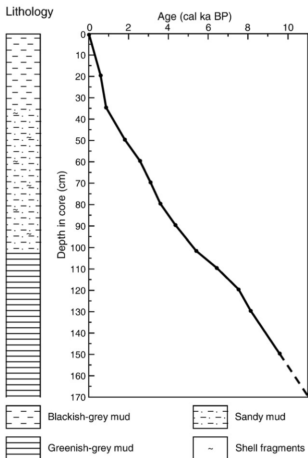
Figure 2. Lithological log and age–depth model of HL06 sediment core recovered in the central part of Hulun Lake. Solid dots represent the mean values of 2\sigma ranges of calibrated ages of corrected radiocarbon dates. Dashed line was derived from two superjacent calibrated ages by linear extrapolation to yield ages for sampled horizons of the lowermost 20-cm sediment core.
