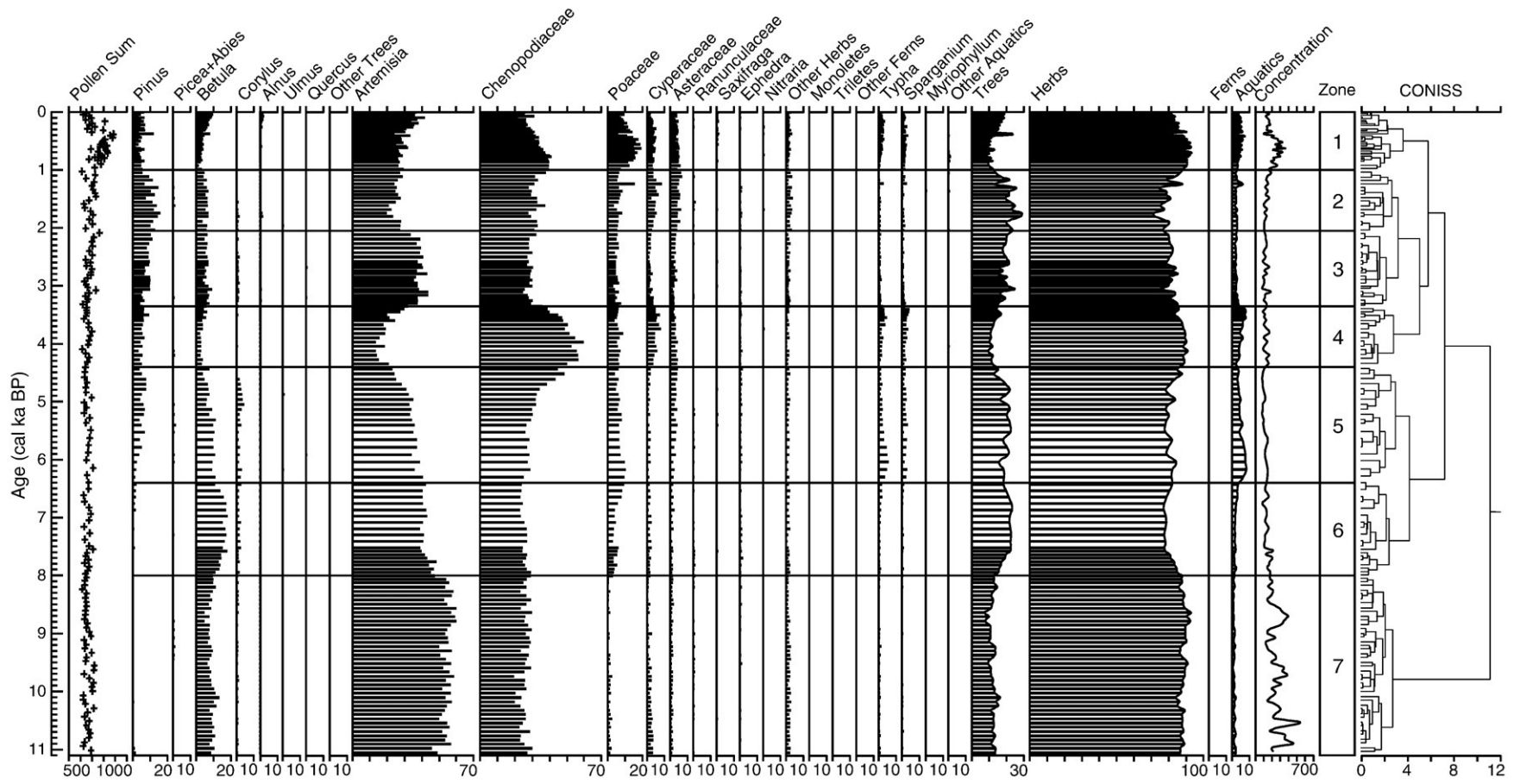
Figure 3. Percentage pollen diagram of HL06 sediment core spanning the last ca. 11,000 yr. Pollen concentrations are expressed in \times 10^3 grains g^{-1} . Cluster analysis (CONISS) is based on the total sum of squares. The chronology was derived from the age-depth model with the reservoir-age corrected.
