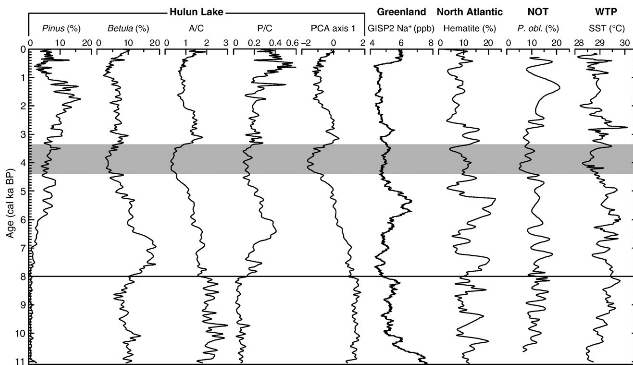
Figure 6. Correlation of Pinus and Betula percentages, Artemisia /Chenopodiaceae (A/C) and Poaceae /Chenopodiaceae (P/C) ratios and pollen PCA axis 1 from Hulun Lake with sea-salt sodium flux ( \text{Na}^+ , ppb) from Greenland GISP2 (Mayewski et al., 1997), hematite-stained grain concentration (hematite, %) from the North Atlantic (Bond et al., 2001), Pulleniatina obliquiloculata abundance ( P. obl. , %) from the northern Okinawa Trough (NOT) (Jian et al., 2000) and sea surface temperature (SST, °C) from the western tropical Pacific (WTP) (Stott et al., 2004). Horizontal line indicates the onset of East Asian summer monsoon intensification during the Holocene. Shaded bar marks the interval of a drastic decline in the summer monsoon precipitation during the middle Holocene.
