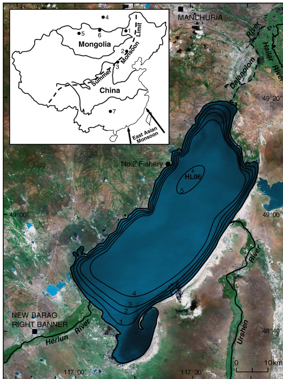
Figure 1. Map of Hulun Lake (from http://maps.google.com ) showing the location of HL06 sediment core. The bathymetric survey of the lake was conducted in July 2005 with an FE-606 Furuno Echo Sounder (contours in meters). In the inset, the current northern limit of the East Asian summer monsoon (dashed line) and the locations of lakes and Dongge Cave (solid circles) mentioned in the text are shown. 1, Hulun Lake; 2, Dali Lake; 3, Daihai Lake; 4, Lake Baikal; 5, Lake Telmen; 6, Gun Lake; 7, Dongge Cave.
