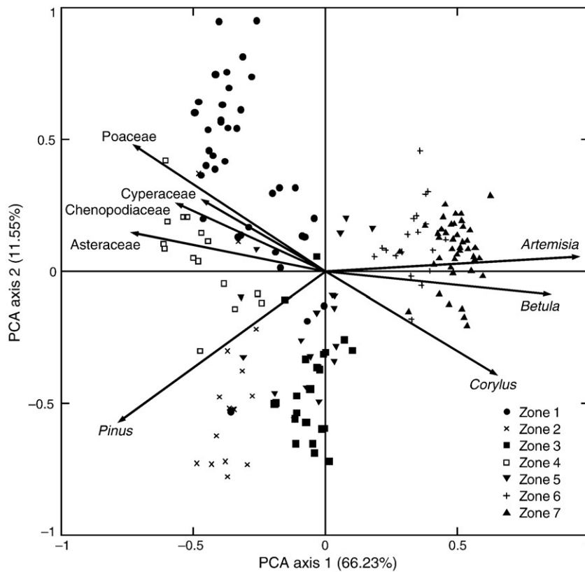
Figure 4. PCA ordination of eight pollen taxa with percentages >3% in any sample and the total pollen data of HL06 sediment core recovered in the central part of Hulun Lake. Eigenvalues of the first four axes are 0.6623, 0.1155, 0.0970 and 0.0575, respectively. The first and second axes capture 77.78% of the total variance within the data set.
