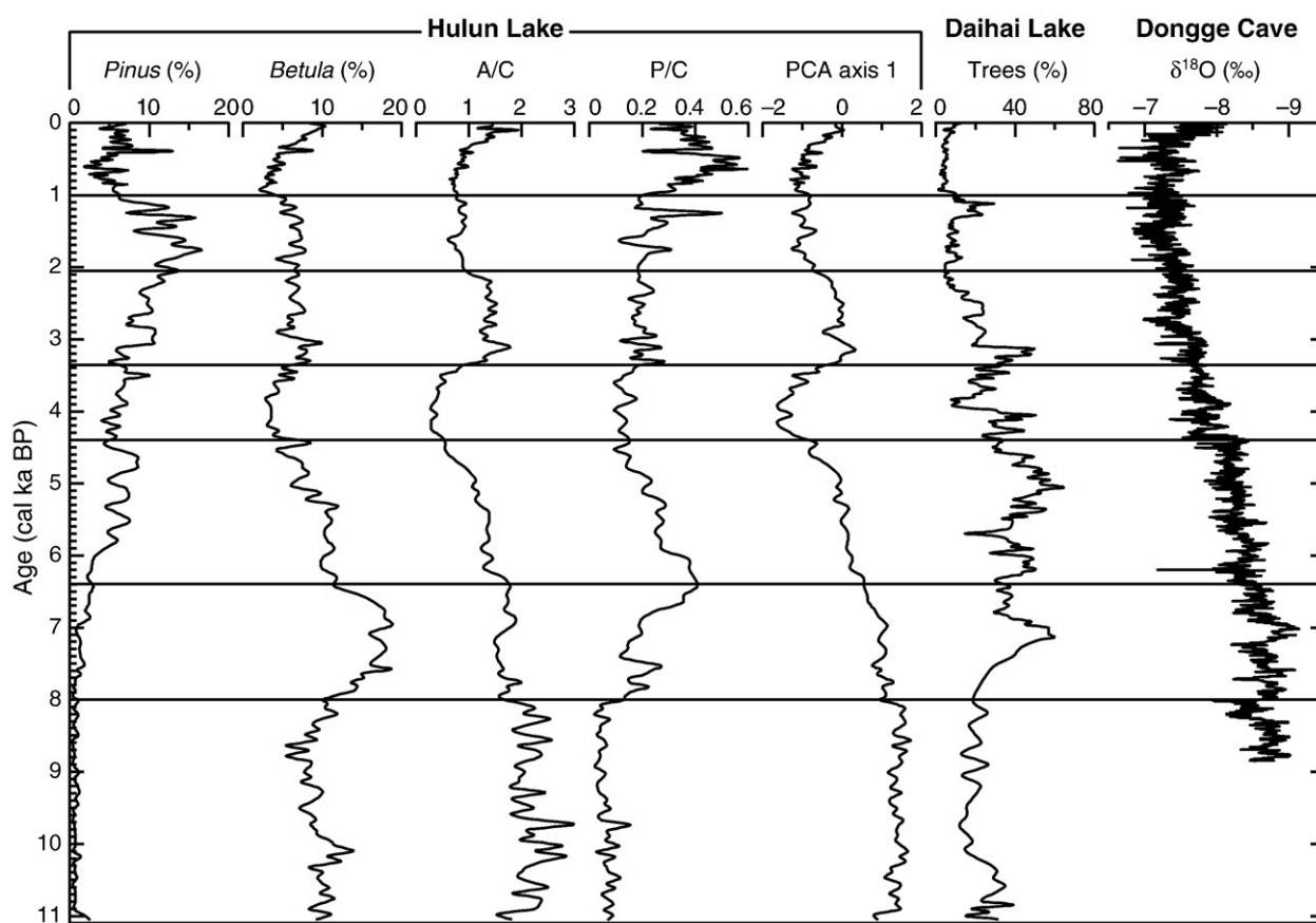
Figure 5. Percentages of Pinus and Betula , ratios of Artemisia to Chenopodiaceae (A/C) and Poaceae to Chenopodiaceae (P/C) and pollen PCA axis 1 of HL06 sediment core spanning the last ca. 11,000 yr, compared with tree pollen percentage of Daihai Lake sediments (Xiao et al., 2004) and δ 18 O of Dongge Cave stalagmite (Wang et al., 2005). Horizontal lines bracket the stages characterizing the pattern of changes in the vegetation and climate over the Hulun Lake region during the Holocene.
