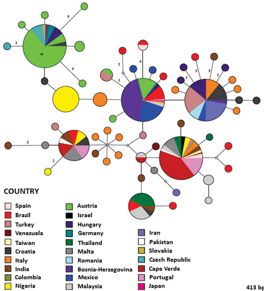
Fig. 3. Median Joining (MJ) haplotype network of the 18S rRNA gene (413 bp) of Hepatozoon canis . Colours indicate different geographic locality and the circle size in the network denotes the number of individuals sharing the same haplotype. Numbers along the branches indicate the number of substitutions between haplotypes. An asterisk (*) in the circle represents sequences (haplotypes) obtained in the present study.
