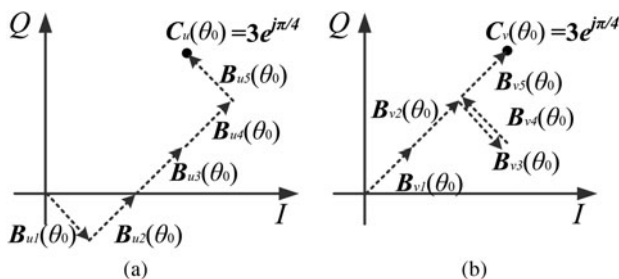
Fig. 5. Illustration example of two vector paths derived from two different excitation settings.
