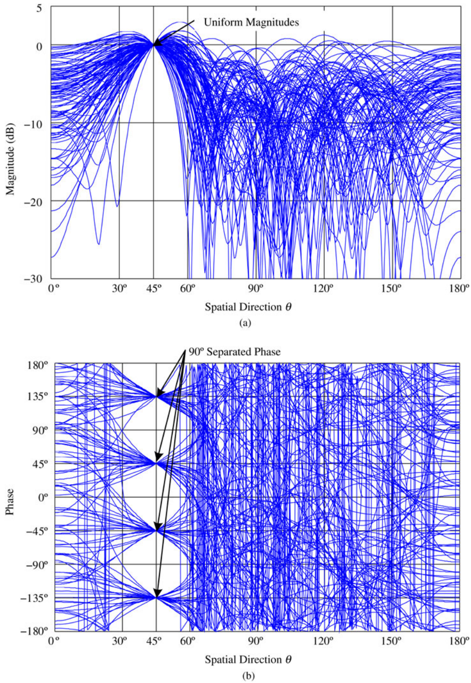
Fig. 6. Simulated far-field (a) magnitude and (b) phase patterns of the 5-element dynamic QPSK DM transmitter array for 100 random QPSK symbols with circularly symmetric independent and identically distributed complex Gaussian distributed v_p ( \sigma_v^2 = 0.8 ).
