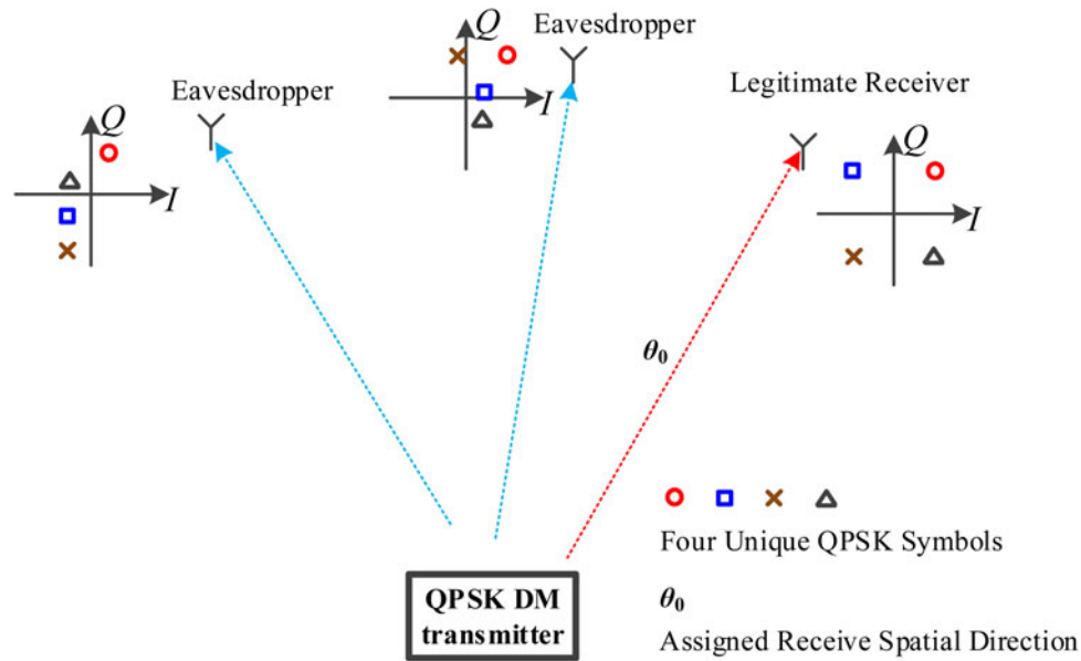
Fig. 1. Illustration of the major properties of a quadrature phase-shift keying (QPSK) directional modulation (DM) system. Along a pre-specified direction \theta_0 , a usable constellation is formed. Away from the desired direction the constellations are scrambled.
