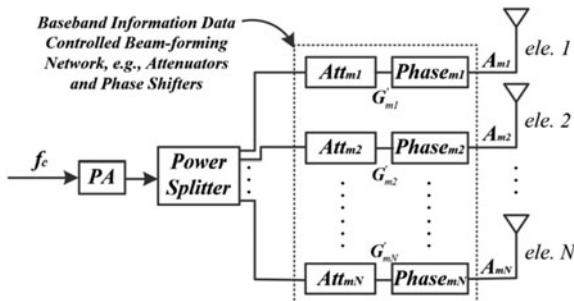
Fig. 3. Generic analog active DM transmitter architecture [10].
