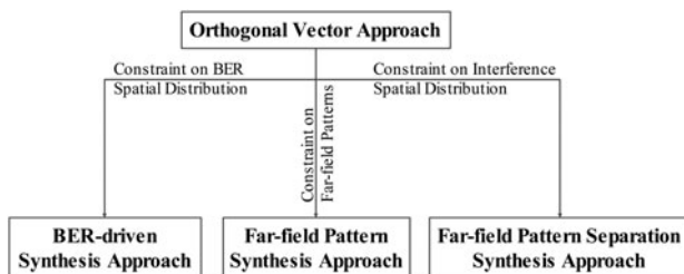
Fig. 8. Relationships among the four DM synthesis approaches.
