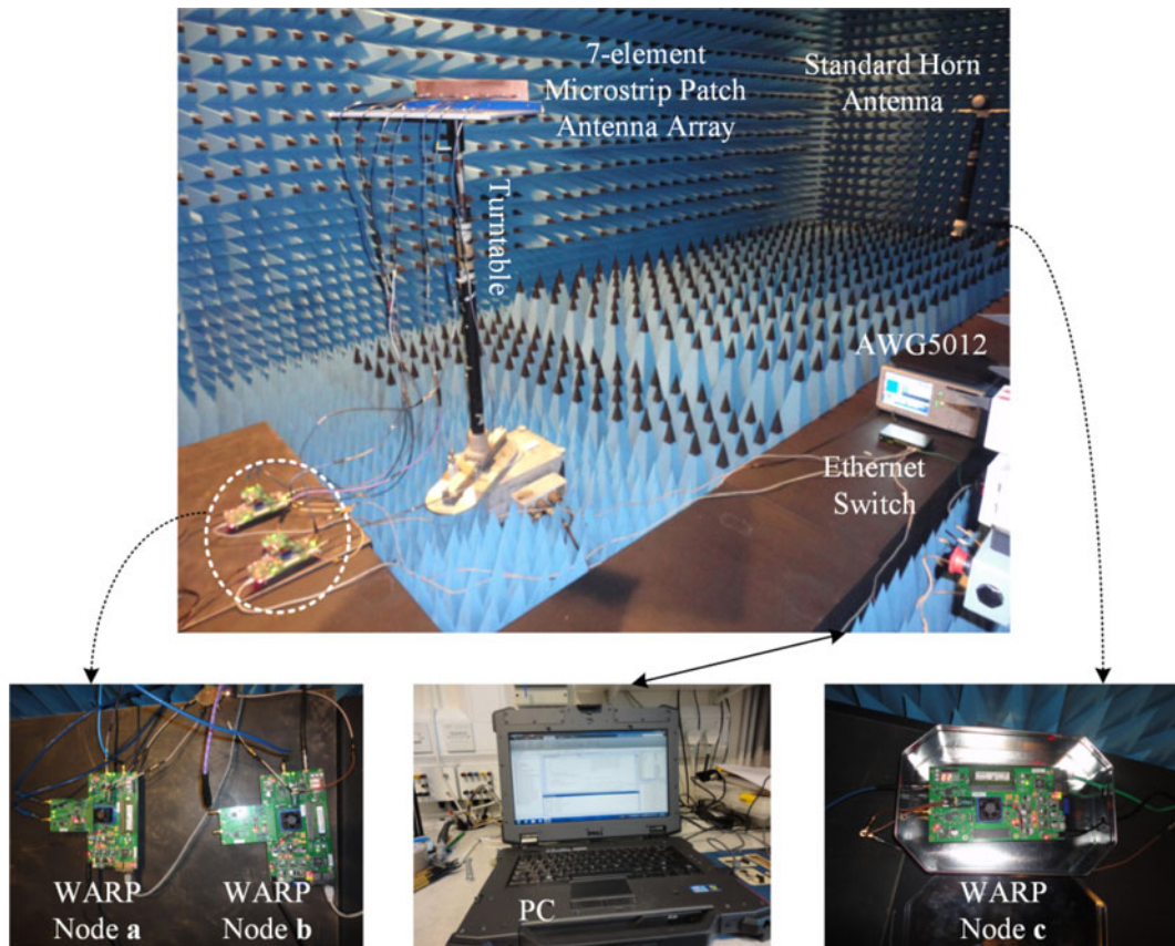
Fig. 10. Photographs of the digital DM experiment [43].
