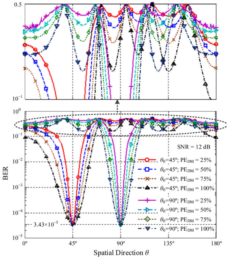
Fig. 7. Simulated bit error rate spatial distributions in dynamic QPSK DM systems with different PE_{DM} s for 45^\circ and 90^\circ secure communications. Signal to noise ratio is set to 12 dB.
