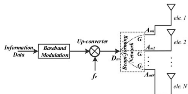
Fig. 2. Conventional “non-DM” transmitter array architecture [10].
