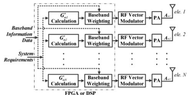
Fig. 4. Generic digital DM transmitter architecture [10].
