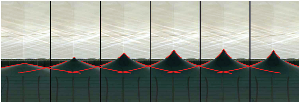
Figure 18. Example of calibrated image edge detection, showing a series of images from Exp. 40 with overlaid red lines showing the detected edges in each image.
