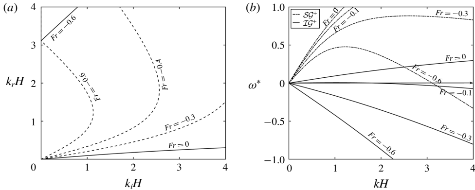
FIGURE 8. (a) Different combinations of k_r on SG^+ such that k_i is on IG^+ for high values of negative Fr for the case of shear in the lower layer. Here R = 0.95 and h_u/h_l = 1/3 . For solid lines, k_b = |k_i - k_r| and for dashed lines, k_b = k_i + k_r . (b) Dispersion relation for negative Fr . Here solid lines represent IG^+ modes and dashed lines represent SG^+ .
