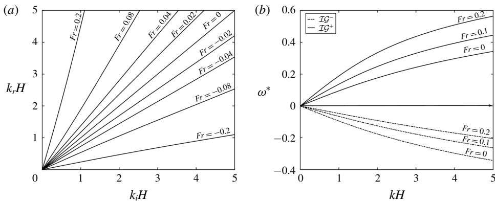
FIGURE 9. (a) Different combinations of k_r on IG^- such that k_i is on IG^+ , for various values of Fr \equiv U_u/\sqrt{gH} when shear is in the upper layer. Here U_l = U_b = 0 , R = 0.95 and h_u/h_l = 1/3 . (b) Dispersion relations for the same case for three values of Fr .
