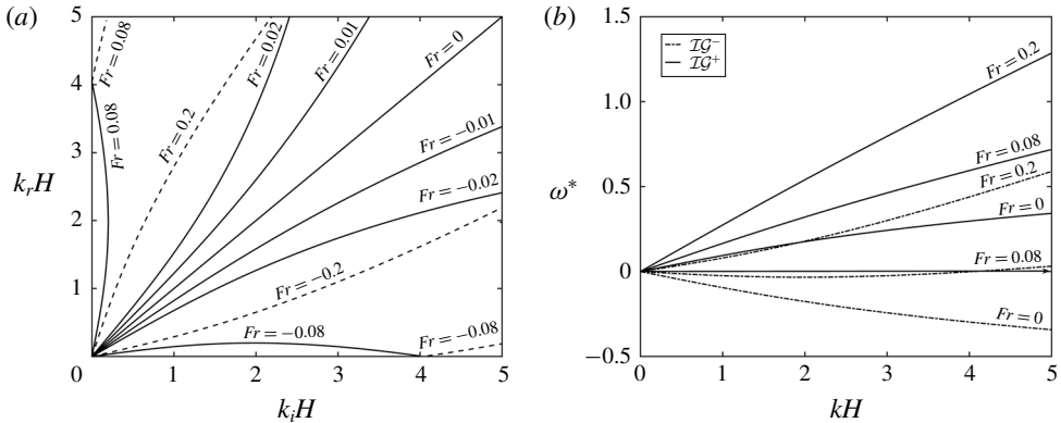
FIGURE 4. (a) Different combinations of k_r on \mathcal{IG}^- such that k_i is on \mathcal{IG}^+ , for various values of Fr when shear is in the lower layer. Here R = 0.95 and h_u/h_l = 1/3 . For solid lines, k_b = k_i + k_r and for dashed lines, k_b = |k_i - k_r| . (b) Dispersion relations for the same case for three values of Fr . Here solid lines represent \mathcal{IG}^+ modes and dashed lines represent \mathcal{IG}^- .
