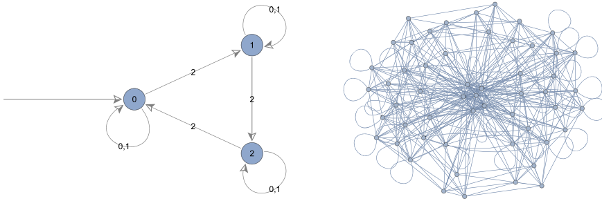
Figure 3: Automata from Example 3.11. The automaton on the left generates the initial condition u , and the automaton on the right generates the spacetime diagram ST_\Phi(u) .
