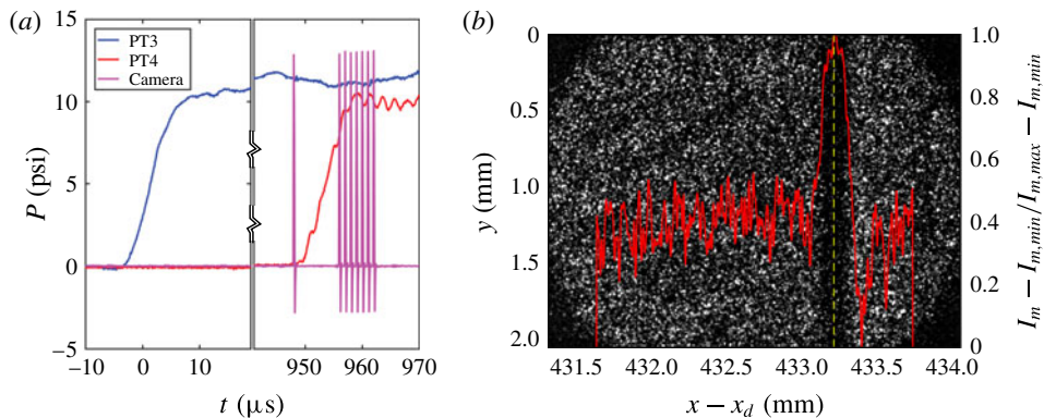
FIGURE 2. (a) Time traces of pressure signals from transducers PT3 and PT4 with the framing camera timing and (b) sample shadowgraph image superposed with the mean intensity profile (red). The shock location is indicated by a dashed line. Image contrast has been enhanced to better show the shock shadowgraph, and the resulting speckle in the image is background noise, not experimental particles.
