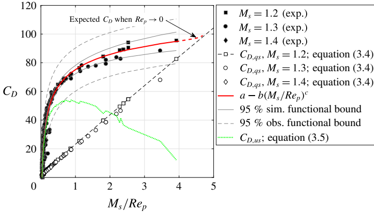
FIGURE 5. Total drag coefficient C_D , quasi-steady ( C_{D,qs} ) and unsteady ( C_{D,us} ) components with respect to M_s/Re_p . The red line is a least-squares fit to the experimental data, C_D = a - b(M_s/Re_p)^c , with a = 167.5 , b = 92.2 and c = -0.18 . The grey solid and dashed lines are simultaneous functional and observational 95% confidence bounds.
