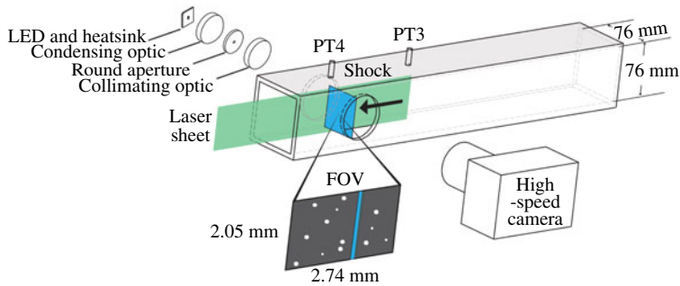
FIGURE 1. Schematic of the test section in the horizontal shock tube. The shock moves from right to left. The inset shows the field of view (FOV) with an example shock position. The camera images the shadowgraph and scattered light from the particles within the laser sheet.
