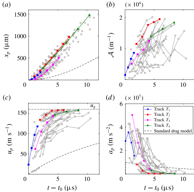
FIGURE 3. (a) Particle location ( x_p ) for M_s = 1.3 experiments obtained from particle tracking with \Delta t = 0.5 \mu\text{s} , 1.0 \mu\text{s} and 2.0 \mu\text{s} , and the corresponding (b) fitting parameter \mathcal{A} (see (3.2)), (c) velocity u_p (see (3.3)) with the post-shock gas velocity ( u_g , -\cdots- ) and (d) acceleration a_p (see (3.1)) obtained from piecewise nonlinear fitting ( -\circ- ). The dashed lines ( - - ) show the values expected from Clift–Gauvin drag (3.4). Four individual particle trajectories, T_1 – T_4 , are highlighted for reference.
