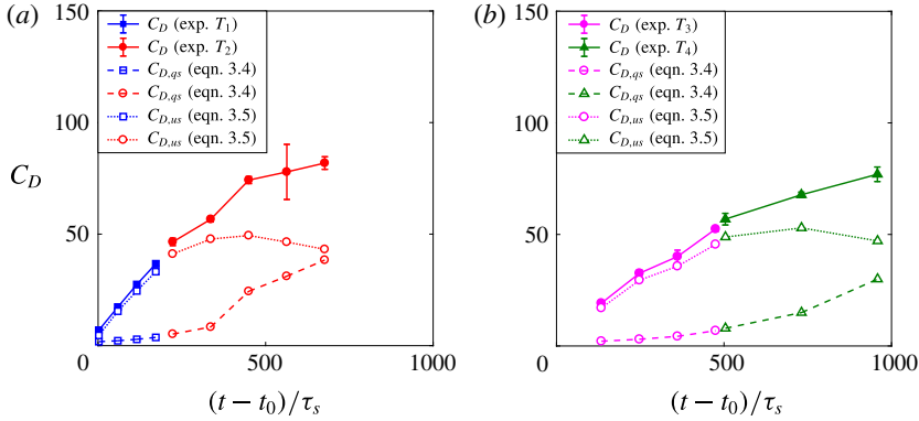
FIGURE 4. The total drag coefficient C_D (solid line), the quasi-steady component C_{D,qs} (dashed line) and the unsteady component C_{D,us} (dotted line) with respect to time normalised by the acoustic time scale ( \tau_s ) for trajectories (a) T_1, T_2 and (b) T_3, T_4 .
