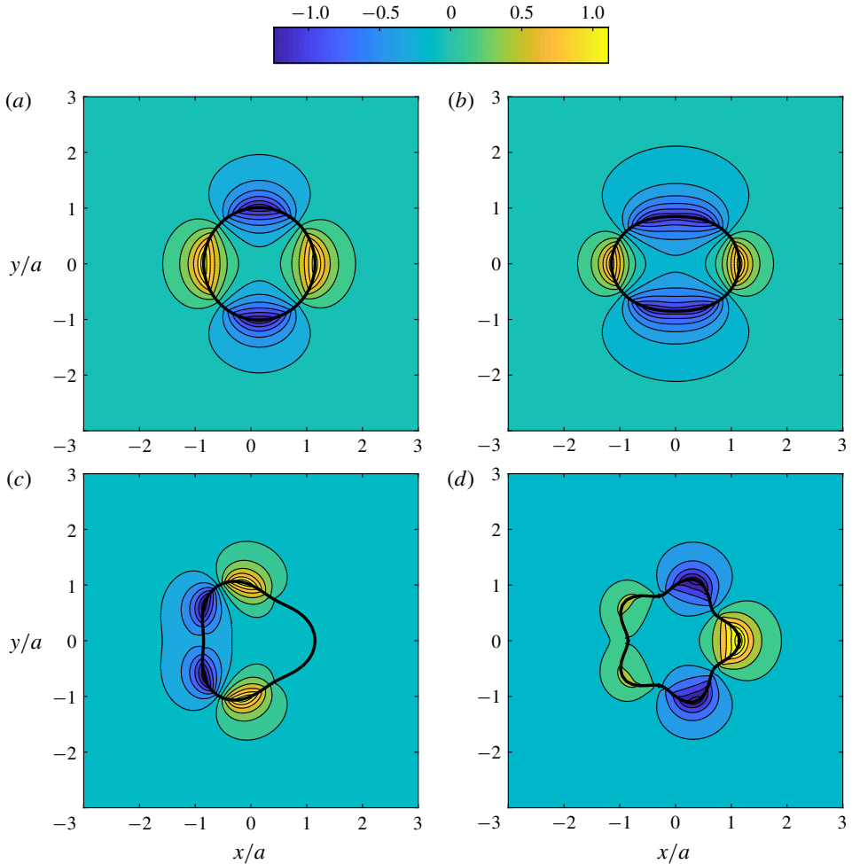
FIGURE 17. (Colour online) The shapes of mode 2 for some strongly lobed geometries when \epsilon = 0.15 at a high frequency of \alpha a \approx 2.5 : (a) N=1 ; (b) N=2 ; (c) N=3 ; (d) N=5 . The thick black solid lines show the lobed vortex sheets.
