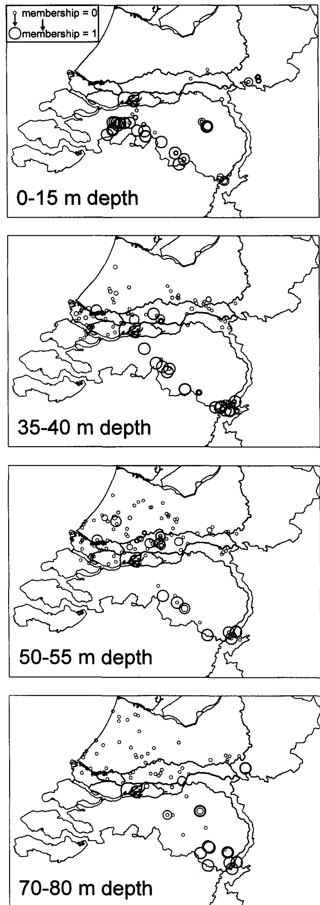
Fig. 4. Spatial patterns of heavy-mineral cluster 1. Point size indicates membership function (see legend).
