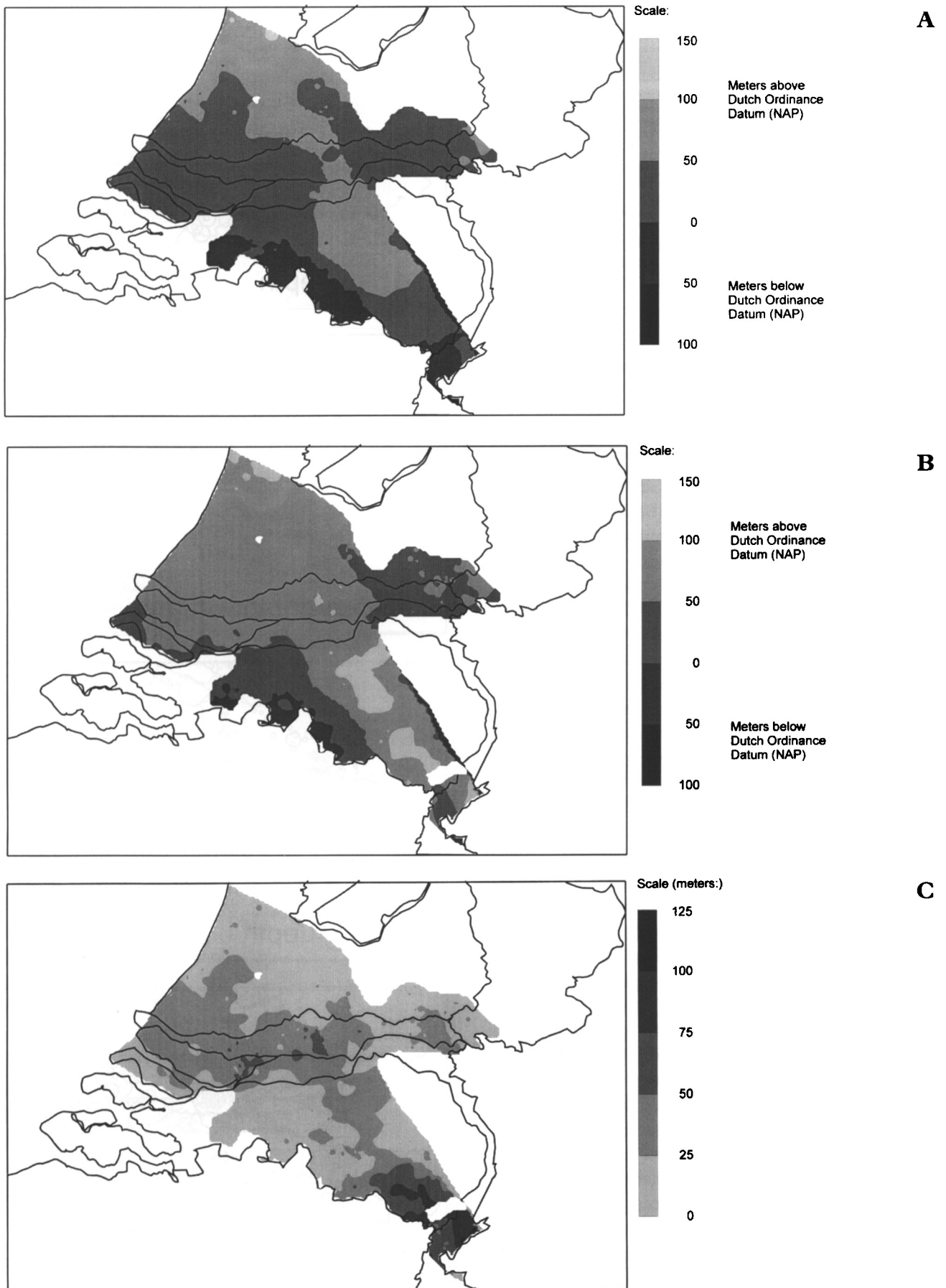
Fig. 2. Boundaries and thickness of the Kedichem Formation. A: upper boundary. B: lower boundary. C: thickness.
