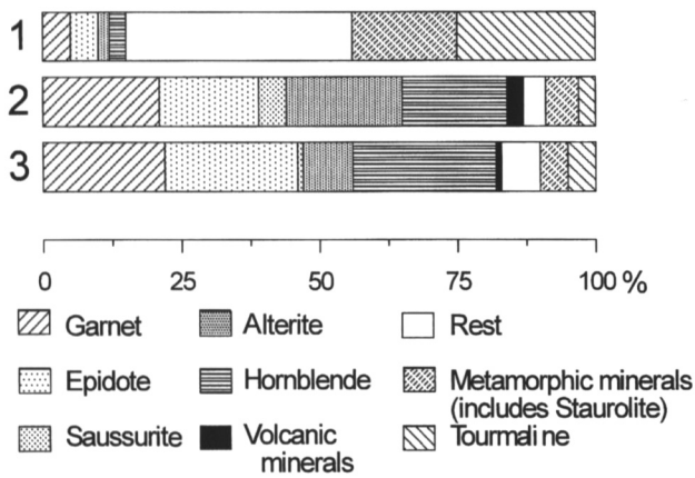
Fig. 3. Heavy-mineral clusters as determined by fuzzy clustering. Cluster 1 consists of stable heavy minerals, whereas clusters 2 and 3 show an association of unstable heavy minerals. The main difference between the two is that cluster 2 has higher alterite contents, whereas cluster 3 shows higher contents of epidote and hornblende.
