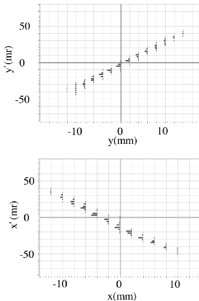
Fig. 6. Horizontal and vertical phase space measurements at the end of the first 10 electrostatic quadrupoles. The lengths of the horizontal bars are proportional to the signal intensity measured at the coordinates of the right end of each bar.
