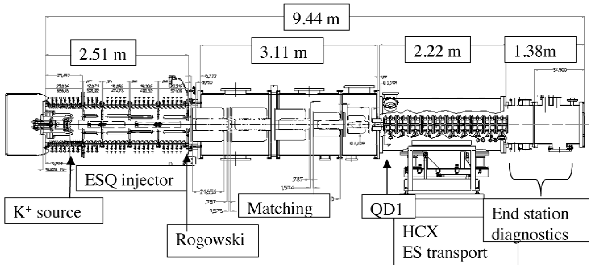
Fig. 1. Elevation view of the present configuration of the HCX experiment.
