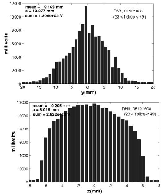
Fig. 3. Vertical (top) and horizontal (bottom) slit-scan profiles at the end of the matching section.
