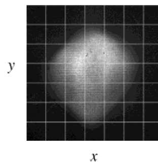
Fig. 7. Intensity distribution of the beam at D-end, measured with a Kapton film. The spacing between the grid lines is 5 mm.
