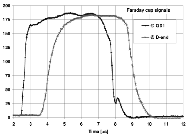
Fig. 5. Capacitive monitor signals from the first and last matching section quadrupoles (QM1 and QM6).
