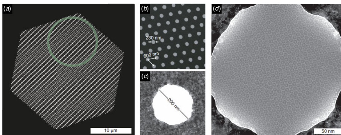
Fig. 5. All-gold specimen supports with sub- \mu\text{m} holes. (a) HexAuFoil grid support designed for movement-free cryoEM imaging. A 3 mm grid contains \sim 800 hexagons, each of which includes more than 5000 holes on a hexagonal lattice. The green line encircles \sim 800 holes. (b) Transmission electron micrograph of the holey gold foil, with arrows delineating the hexagonal lattice. (c) Micrograph of a single empty 200 nm hole. (d) Low-dose transmission electron micrograph of the 223 kDa DPS protein vitrified in the 260 nm holes of a HexAuFoil grid (Naydenova et al. , 2020).
