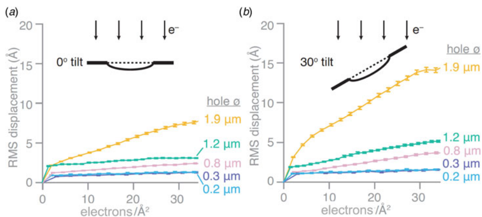
Fig. 6. Beam-induced movement depends on hole diameter. Root mean squared (RMS) displacements of gold particles in vitrified water from movies of all-gold grid holes of different diameters. Displacements are plotted as a function of cumulative electron dose for untilted specimens (a) and specimens tilted in the electron microscope by 30° (b) (Naydenova et al. , 2020).
