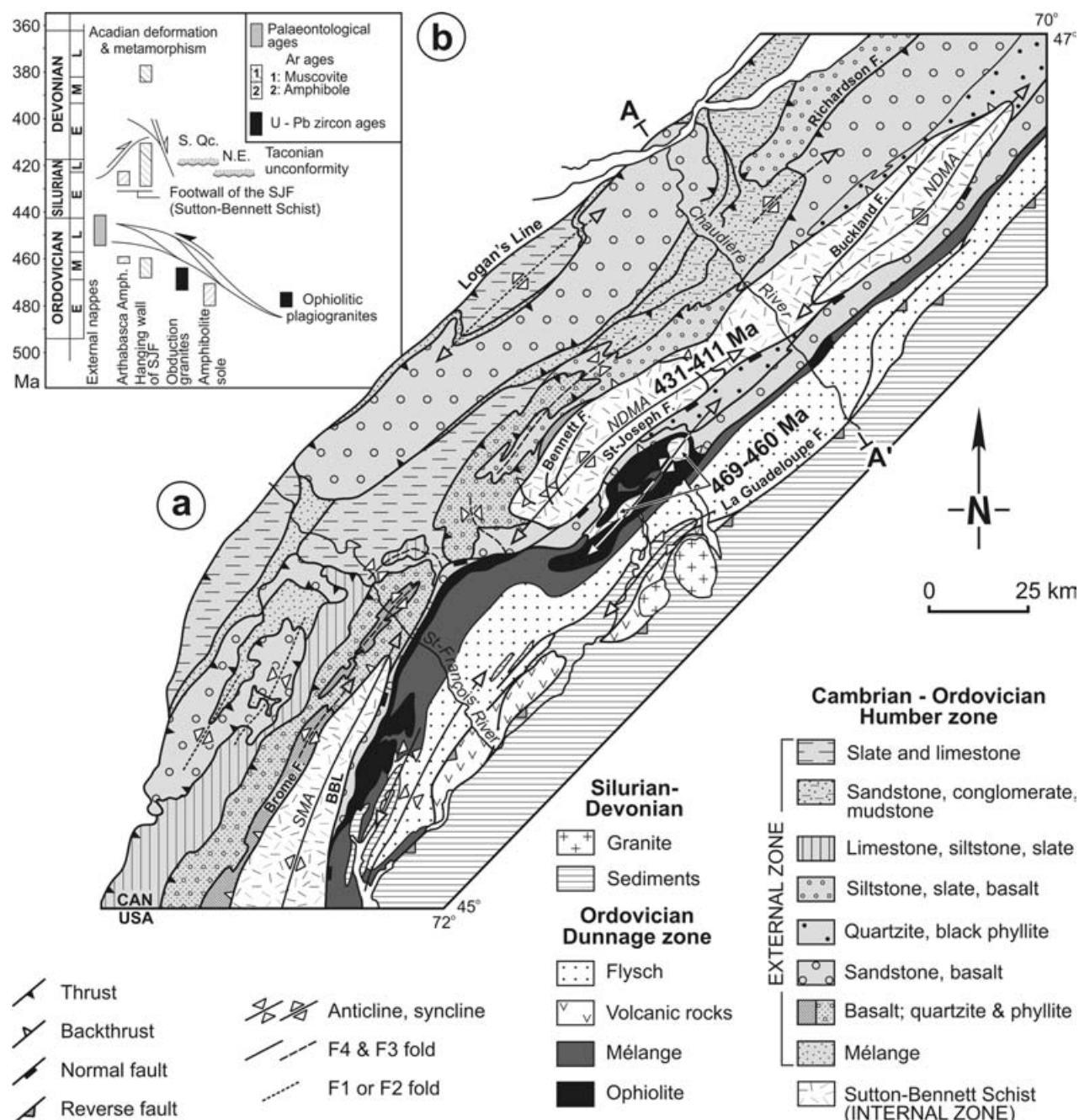
Figure 6. (a) Geological map of the southern Québec Appalachians showing the distribution of Ordovician and Silurian/Early Devonian 40 Ar/ 39 Ar ages for the internal Humber zone on both sides of the Saint-Joseph fault. (b) Diagram illustrating the various geochronological data available in this region. SMA – Sutton Mountains anticlinorium; NDMA – Notre-Dame Mountains anticlinorium; BBL – Baie Verte-Brompton Line; SJF – Saint-Joseph fault; S.Qc. – southern Québec; N.E. – New England. A–A’ – location of the structural profile of Figure 7. See text for details and Figure 1 for location.
