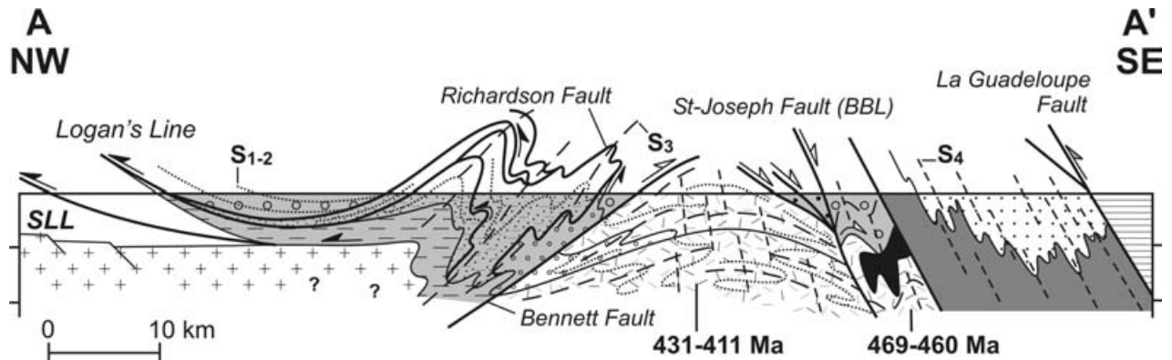
Figure 7. Structural profile of the southern Québec Appalachians illustrating the geometry and kinematics of regional polyphased deformation. The orientation of S_{1-2} , S_3 and S_4 tectonic fabrics as defined by Tremblay & Pinet (1994) are schematically shown. See Figure 6 for legend and location.
