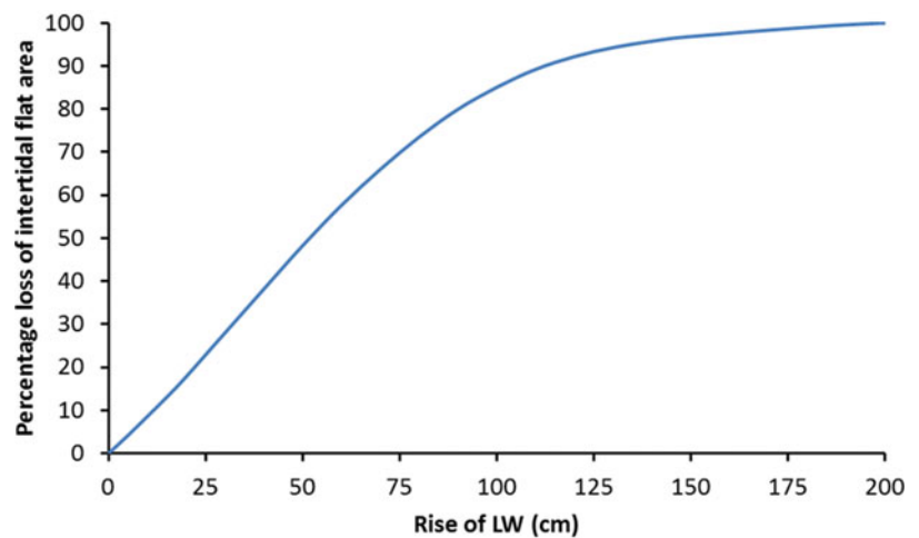
Fig. 11. Relation between loss of intertidal flat area in the Dutch Wadden Sea and rise of the Low Water level, derived on the basis of the most recent hypsometric curve (2012) assuming the present Low Water level at -1\text{ m} NAP.
