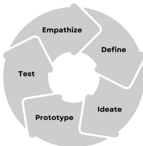
Figure 1 Design thinking.
