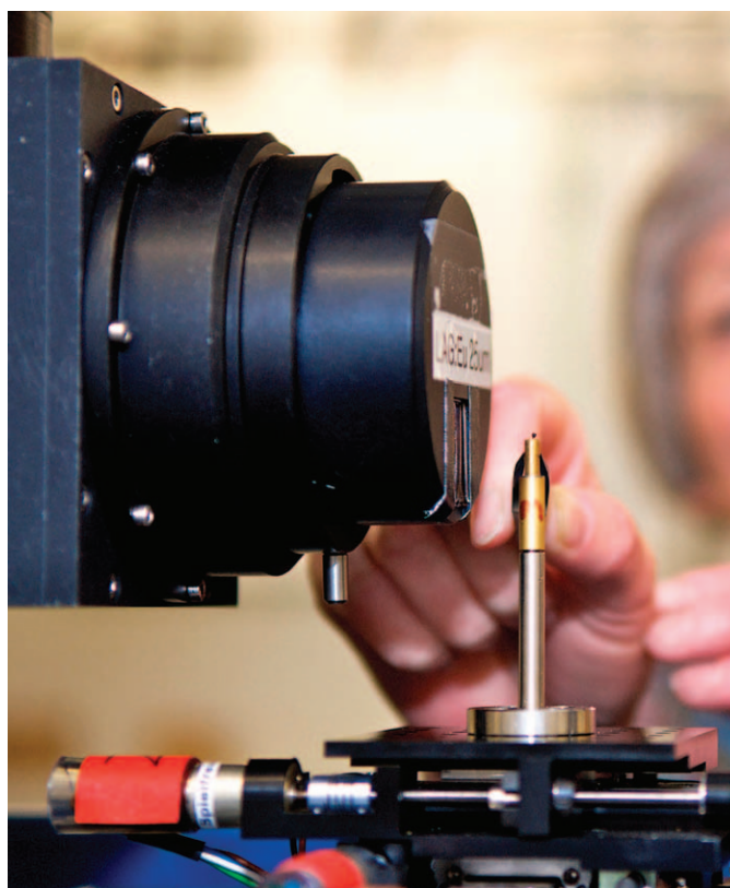
FIGURE 1—Close-up view of the TOMCAT end station showing the sample holder with a fossil flower mounted on a brass stub, 3 mm in diameter, in front of the microscope. (Paul Scherrer Institute photo).
