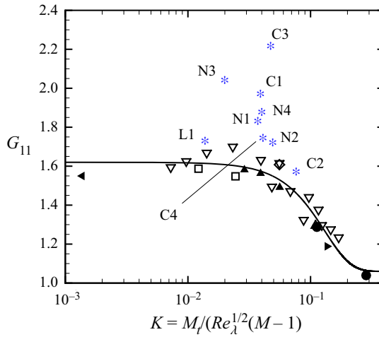
Figure 2. Reynolds stress R_{11} amplification factor G_{11} versus K \equiv M_t/Re_\lambda^{1/2}(M - 1) : current DNS results (*, blue), Lee et al. (1993) ( \blacktriangleright ), Hannappel & Friedrich (1995) ( \diamond ), Barre, Alem & Bonnet (1996) ( \blacktriangleleft ), Lee et al. (1997) ( \square ), Mahesh et al. (1997) ( \nabla ), Jamme et al. (2002) ( \bullet ), Larsson & Lele (2009) ( \Delta ), Boukharfane et al. (2018) ( \blacktriangle ). The solid line is the original proposed fit of Donzis (2012a). Note that the proposed fit has been superseded by the more sophisticated analysis of (Chen & Donzis 2019). It is used here for its simplicity (i.e. lack of Mach number dependence) and for a means of separating the data points visually. Data points should not be expected to collapse completely. Adapted from Donzis (2012a).
