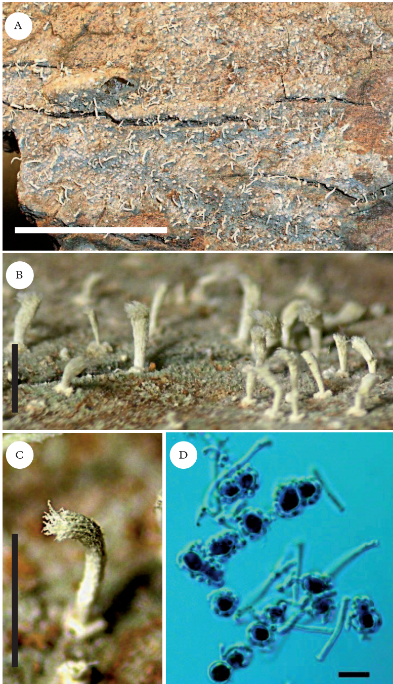
FIG. 1. Nyungwea pallida (type). A, general habit; B, lateral view of the goniocysts-producing stipes; C, lateral view of a single stipe with individual goniocysts visible; D, goniocysts in LCB. Scales: A=10 mm; B=1 mm; C=1 mm; D=10 \mu m.
