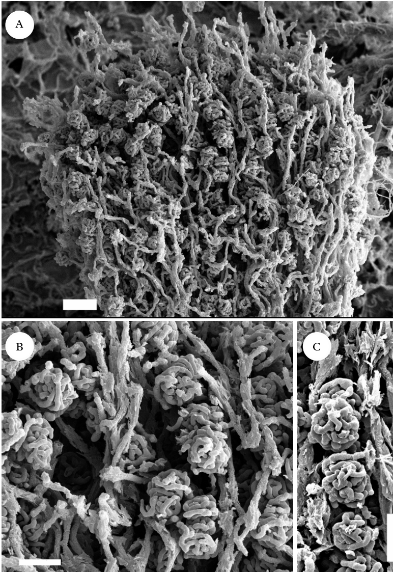
FIG. 2. Nyungwea pallida (type), SEM photographs. A, lateral view of a goniocysts-producing stipe with numerous goniocysts; B & C, detail of chains of goniocysts. Scales: A=20 \mu\text{m} ; B–C=10 \mu\text{m} .
