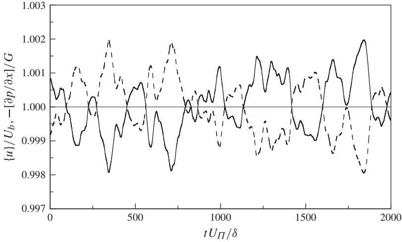
FIGURE 5. Temporal behaviour of the space-mean instantaneous bulk velocity \{u\} (thick solid line) and the space-mean instantaneous pressure gradient -[\partial p/\partial x] (dashed line), normalized with their time-average values U_b and G . The thin horizontal line is the product of the two quantities, proportional to the instantaneous power input, which remains constant during the simulation.
