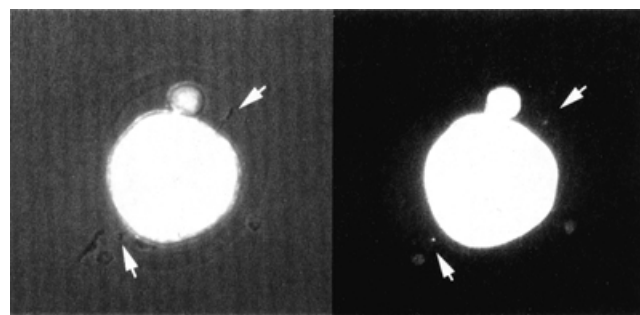
Figure 5 Monobromobimane (mBBr) fluorescence of rat sperm nuclei in the perivitelline space (arrows).
