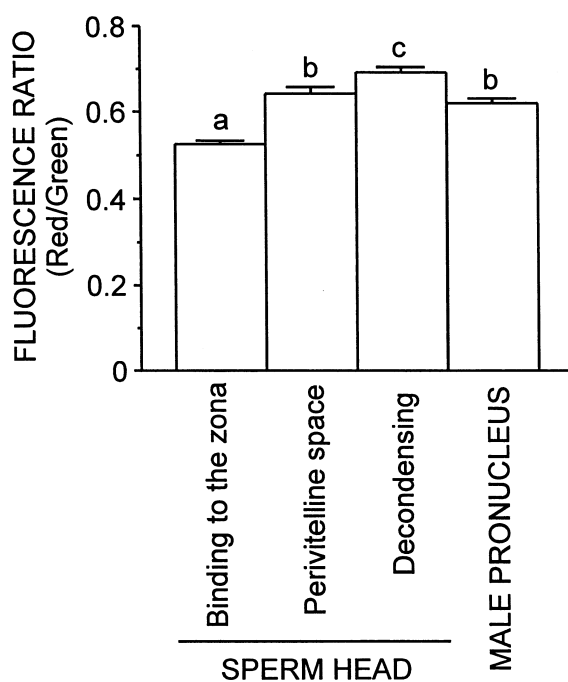
Figure 4 Changes in the acridine orange fluorescence of sperm nuclei during penetration of rat oocytes. The red/green fluorescence ratio of the nucleus was measured by confocal fluorescence microscopy. Bars with different letters differ ( p < 0.05 ).
