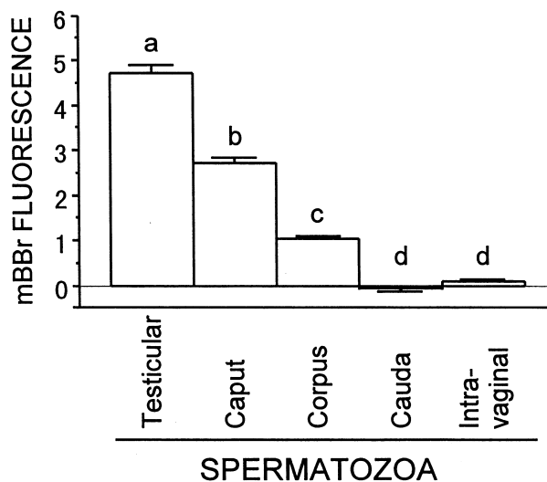
Figure 3 Changes in the monobromobimane (mBBr) fluorescence of rat sperm nuclei during epididymal maturation. The fluorescence intensity of sperm nucleus was measured using an epifluorescence microfluorometer. Bars with different letters differ ( p < 0.05 ).
