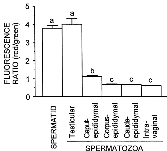
Figure 1 Changes in the acridine orange fluorescence of rat sperm nuclei during maturation. The red/green fluorescence ratio of the nucleus was measured by confocal fluorescence microscopy. Bars with different letters differ ( p < 0.05 ).
