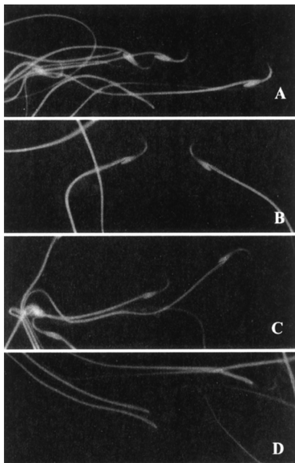
Figure 2 Monobromobimane (mBBr) fluorescence of rat sperm nuclei during epididymal maturation. (A) Testicular spermatozoa; (B) caput-epididymal spermatozoa; (C) corpus-epididymal spermatozoa; (D) cauda-epididymal spermatozoa.
