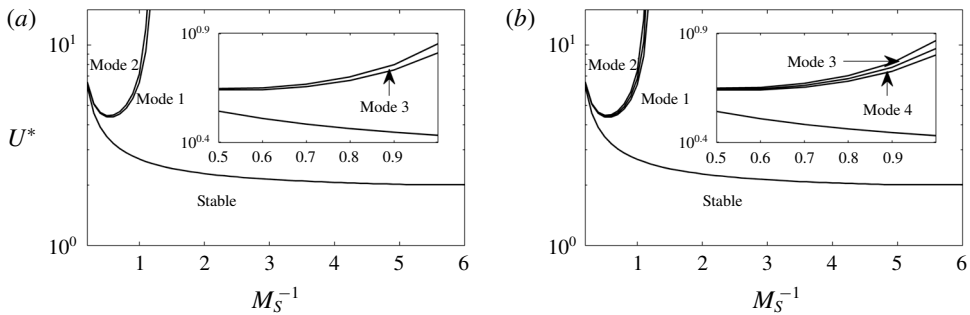
FIGURE 12. (a) Observation of the coupled flapping modes of n=3 and d^*=2 : \eta_{01}/\eta_{03} = 1 , \eta_{02}/\eta_{03} = -p_{31} (mode 1); \eta_{01}/\eta_{03} = 1 , \eta_{02}/\eta_{03} = p_{32} (mode 2); and \eta_{01}/\eta_{03} = -1 , \eta_{02} = 0 (mode 3). (b) Observation of the coupled flapping modes of n=4 and d^*=2 : \eta_{01}/\eta_{04} = -1 , \eta_{02}/\eta_{03} = -1 , \eta_{01}/\eta_{02} = -p_{41} (mode 1); \eta_{01}/\eta_{04} = 1 , \eta_{02}/\eta_{03} = 1 , \eta_{01}/\eta_{02} = p_{42} (mode 2); \eta_{01}/\eta_{04} = -1 , \eta_{02}/\eta_{03} = -1 , \eta_{01}/\eta_{02} = p_{43} (mode 3); and \eta_{01}/\eta_{04} = 1 , \eta_{02}/\eta_{03} = 1 , \eta_{01}/\eta_{02} = -p_{44} (mode 4).
