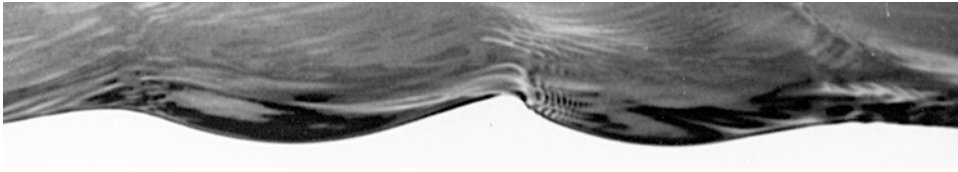
Figure 1. Experimental picture showing parasitic ripples located near the crests of steep gravity waves from Ebuchi, Kawamura & Toba (1987) (reproduced with permission).
