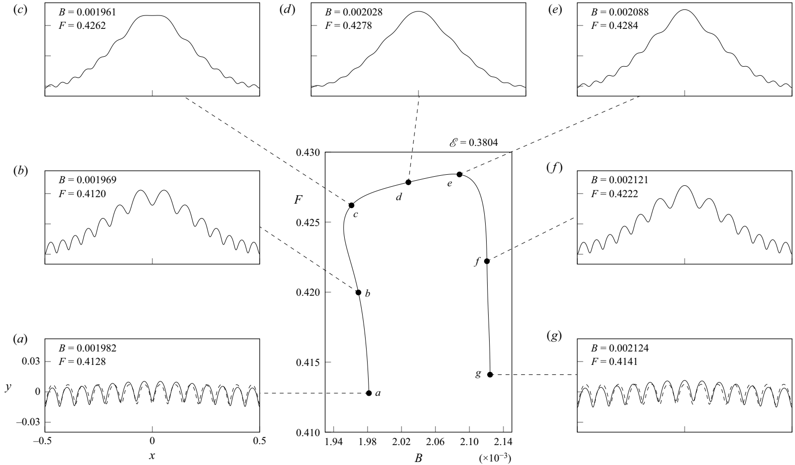
Figure 6. A single finger of solutions, G_{13 \rightarrow 14} , is displayed in the (B, F) -plane for a value of \mathcal{E} = 0.3804 . The dashed profiles in (a) and (g) are solutions from branches S_{13} and S_{14} near the bifurcation point. The (b)–(g) axis limits are the same as inset (a).
