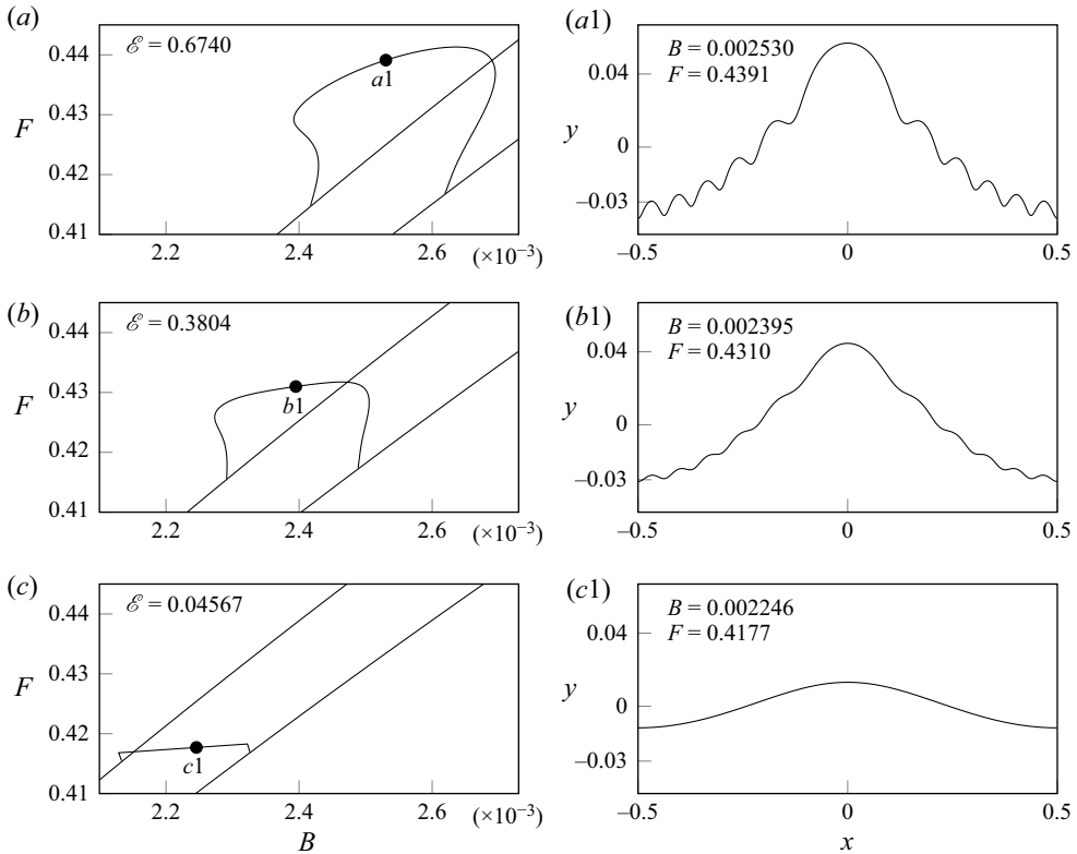
Figure 10. Shown in the left subplots are the fingers G_{11 \rightarrow 12} and the side branches S_{11} and S_{12} , plotted in the (B, F) -plane, for (a) \mathcal{E} = 0.67 ; (b) \mathcal{E} = 0.3804 ; (c) \mathcal{E} = 0.046 . Example solutions, near the tops of the fingers, are shown in the corresponding right subplots labelled (a1), (b1) and (c1).
