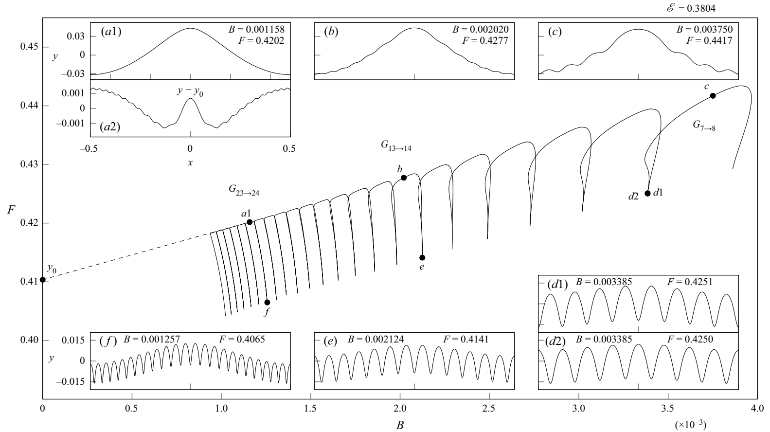
Figure 8. Multiple fingers G_{7 \rightarrow 8} to G_{28 \rightarrow 29} are shown to form one connected branch in the (B, F) -plane at fixed \mathcal{E} = 0.3804 . The (b) – (c) axes limits are the same as inset (a1) and the (e) – (d) limits are the same as inset (f) .
