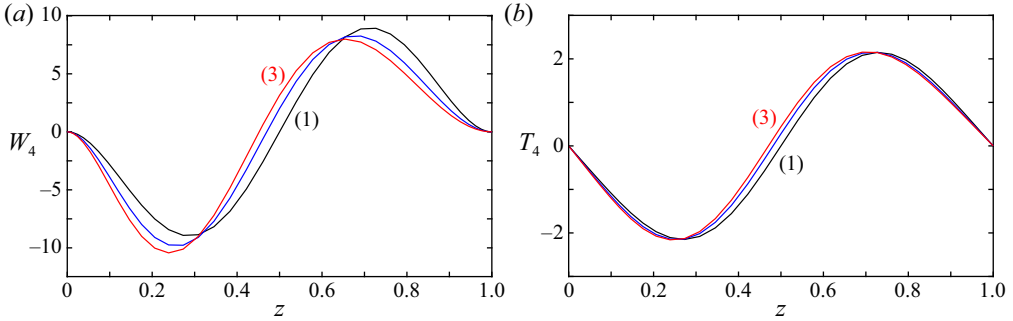
FIGURE 7. Modes factor of \exp(ik_p \cdot r) at Pr = 50 and different values of r : (1) r = 1 ; (2) r = 2 and (3) r = 3 .
