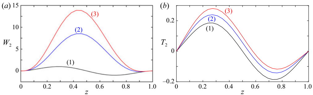
FIGURE 5. First harmonic of the fundamental at Pr = 50 and different values of the viscosity ratio: (1) r = 1 ; (2) r = 2 and (3) r = 3 .
