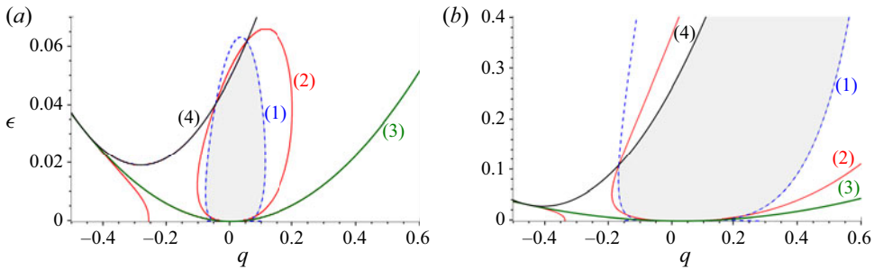
FIGURE 18. Hexagon stability diagram for a shear-thinning fluid with \alpha = 10^{-4} at Pr = 50 and two different values of the viscosities ratio: (a) r = 1.5 and (b) r = 2.5 . Hexagons are stable inside the grey area.
