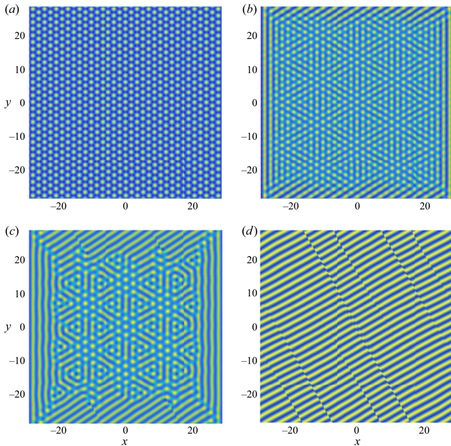
FIGURE 24. Initial condition ( \mathcal{P}_2 ): hexagons with q = 0.55 , \epsilon = 0.3 , r = 2.5 , \alpha = 10^{-4} and Pr = 50 . The reconstructed vertical velocity w is shown at different times: (a) t = 0 , (b) t = 2 , (c) t = 10 and (d) t = 100 .
