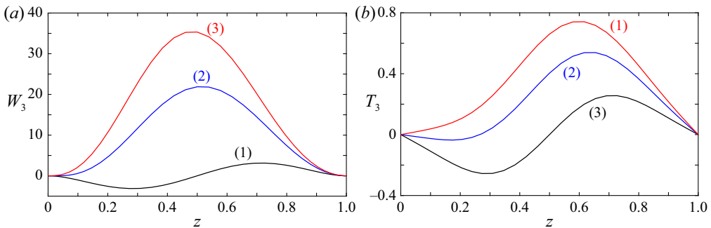
FIGURE 6. Modes factor of A_p A_q^* \exp(i(k_p - k_q)z) at Pr = 50 and different values of r : (1) r = 1 ; (2) r = 2 and (3) r = 3 .
