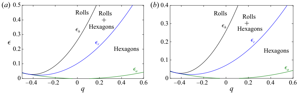
FIGURE 14. Amplitude stability curves in the (\epsilon, q) plane at r = 2.5, Pr = 50 and two different values of \alpha : (a) \alpha = 0 Newtonian fluid, (b) \alpha = 10^{-4} Carreau fluid.
