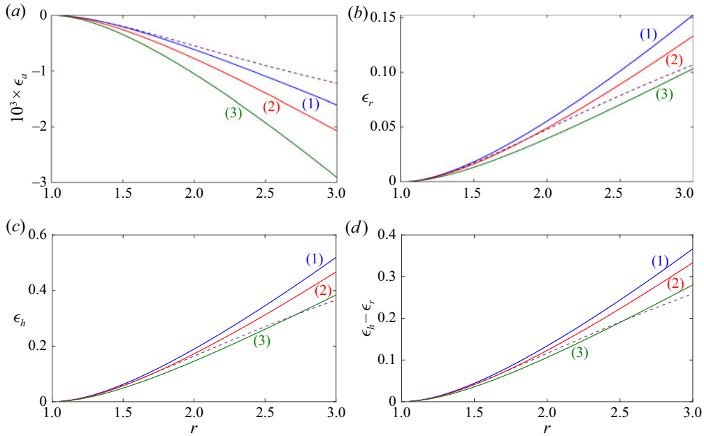
FIGURE 16. Variations of \epsilon_a , \epsilon_r , \epsilon_h and (\epsilon_h - \epsilon_r) versus r for three values of the shear-thinning degree \alpha . The Prandtl number is fixed, Pr = 50 . (1) Newtonian fluid, \alpha = 0 ; (2) Carreau fluid with \alpha = 0.5 \cdot 10^{-4} ; (3) Carreau fluid with \alpha = 10^{-4} . The dashed line is the correlation proposed par Busse (1967) for a Newtonian fluid, assuming a linear variation of the viscosity with temperature.
