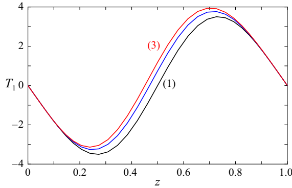
FIGURE 4. Modification of the conductive temperature profile at Pr = 50 and different values of the viscosity ratio: (1) r = 1 ; (2) r = 2 and (3) r = 3 .
