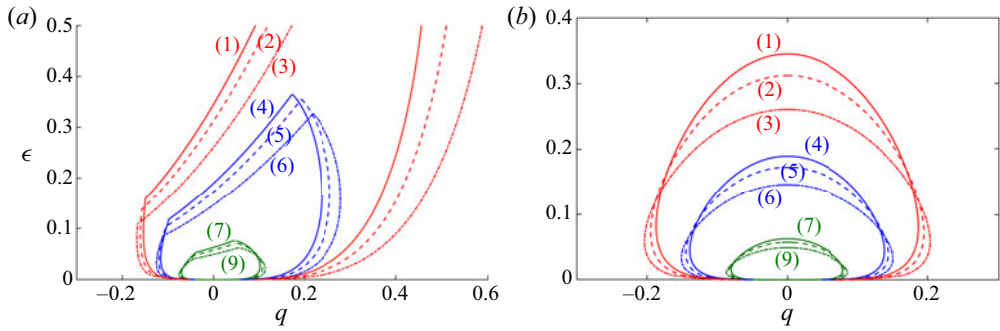
FIGURE 19. Influence of shear-thinning effects and viscosities ratio on the hexagons stability diagram at Pr = 50 . (a) Spatial non-variational terms in (4.22) are taken into account, (b) \alpha_1 = \alpha_2 = 0 . Curves (1), (4) and (7) correspond to a Newtonian fluid and three different values of r : 2.5, 2.0, 1.5, respectively. Curves (2), (5) and (8) correspond to a shear-thinning fluid with \alpha = 5 \times 10^{-5} . Curves (3), (6) and (9) correspond to a shear-thinning fluid with \alpha = 10^{-4} .
