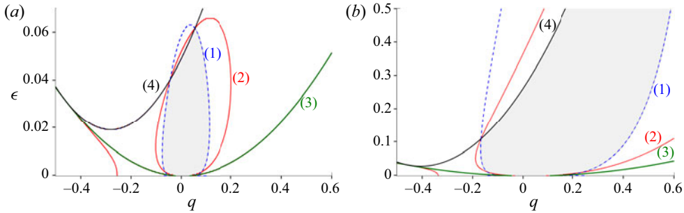
FIGURE 17. Hexagon stability diagram for a Newtonian fluid at Pr = 50 and two different values of the viscosities ratio: (a) r = 1.5 and (b) r = 2.5 . Hexagons are stable inside the grey area. Curve (1): D_{\perp} = 0 , curve (2) D_{\parallel} = 0 , curve (3) bifurcation from the conductive state to convection with hexagons, curve (4) bifurcation from hexagons to rolls.
