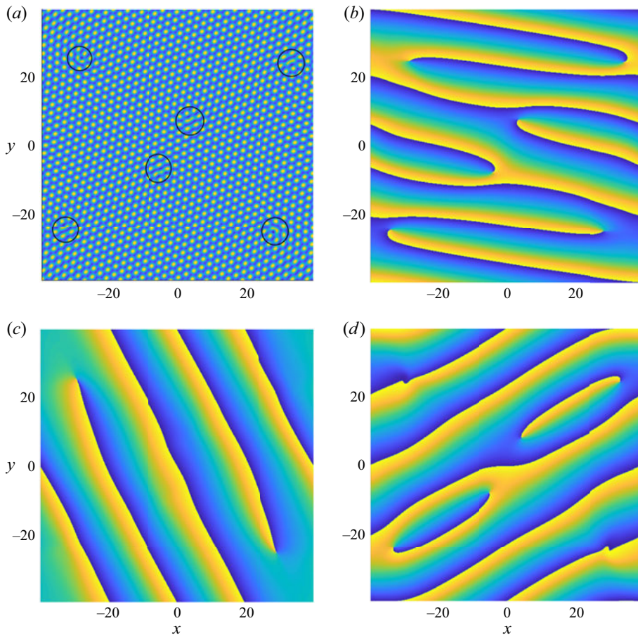
FIGURE 23. Initial condition ( \mathcal{P}_1 ): hexagons with q = 0.45 , \epsilon = 0.1 , r = 2.5 , \alpha = 10^{-4} and Pr = 50 . (a) Contours of the vertical velocity w = \sum_{i=1}^3 A_i \exp(\mathbf{i} \mathbf{k}_{c,i} \cdot \mathbf{x}) + \text{c.c.} at t = 1000 ; (b) phase of A_1 ; (c) phase of A_2 and (d) phase of A_3 .
