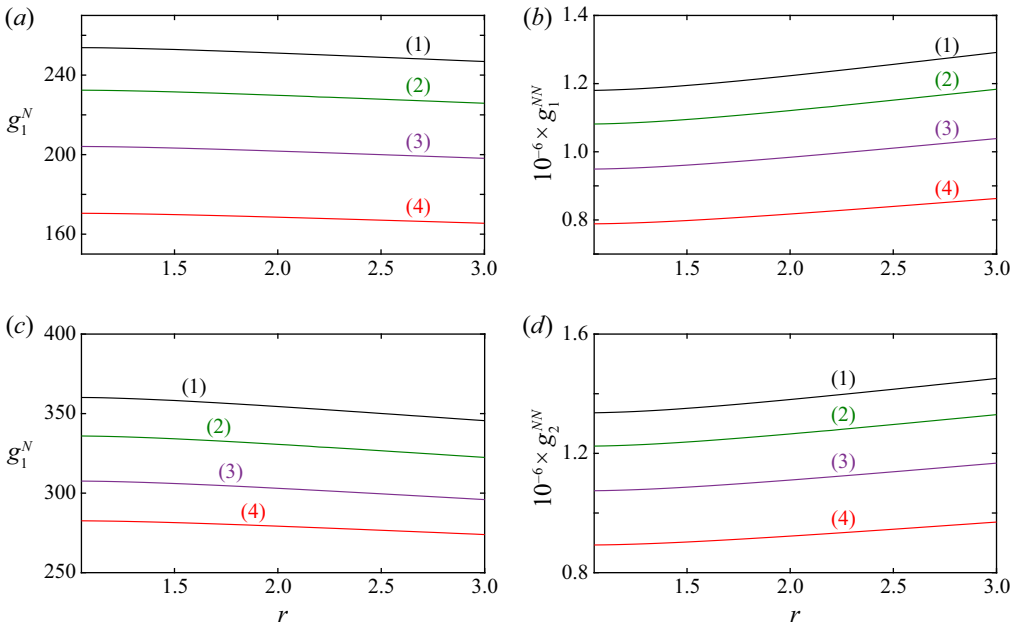
FIGURE 10. (a) ‘Newtonian’ and (b) non-Newtonian contribution to the first Landau coefficient and to the cross-saturation coefficient (c) and (d), respectively, as a function of r for different values of Pr . (1) Pr = 50 ; (2) Pr = 5 ; (3) Pr = 2 ; (4) Pr = 1 .
