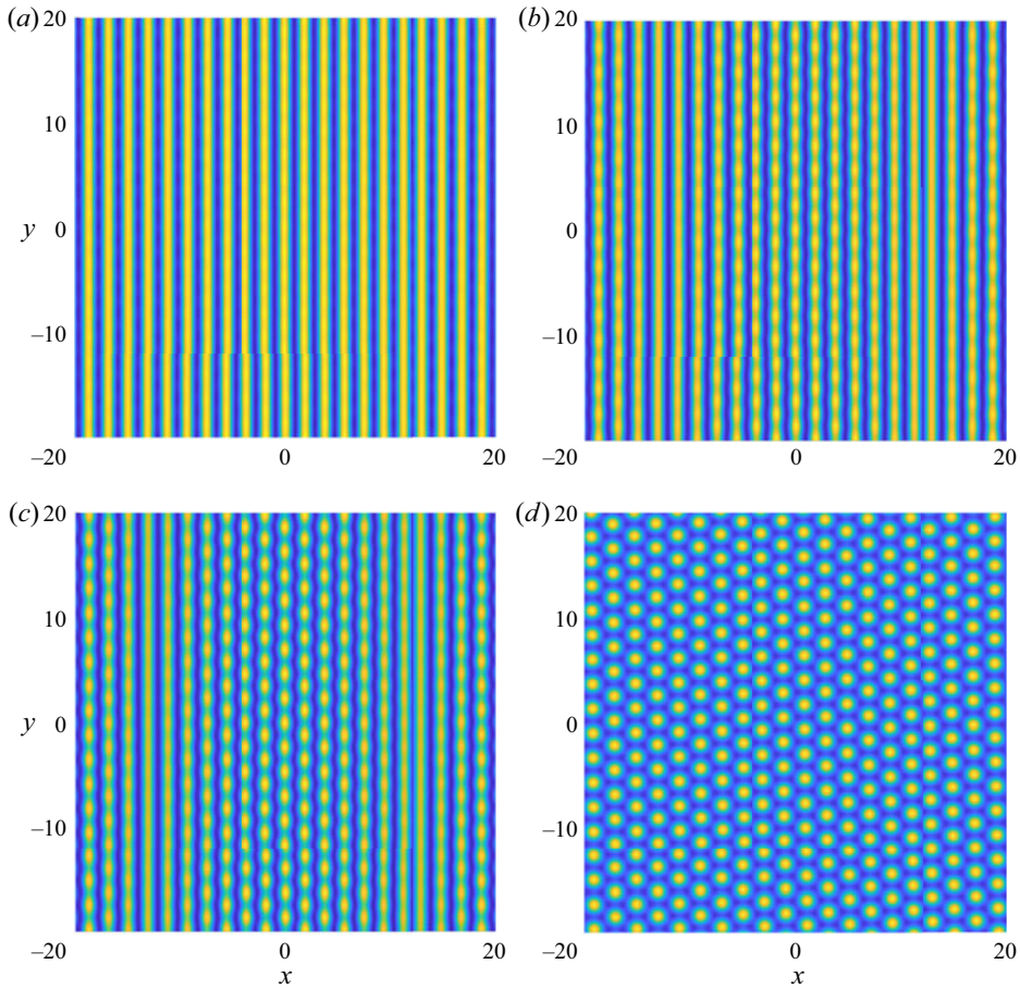
FIGURE 25. Initial condition ( \mathcal{P}_3 ): rolls with q = 0.25 , \epsilon = 0.1 , r = 2.5 , \alpha = 10^{-4} and Pr = 50 . The reconstructed vertical velocity w is shown at different times: (a) t = 0 , (b) t = 11 , (c) t = 15 and (d) t = 2000 .
