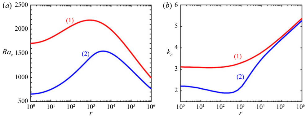
FIGURE 1. Exponential fluid. Critical Rayleigh number (a) and critical wavenumber (b) as a function of the viscosity ratio. (1) NSBC, (2) SFBC.
