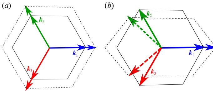
FIGURE 12. (a) Dilatation and (b) distortion of hexagonal pattern (Echebarria & Perez-Garcia 2001).
