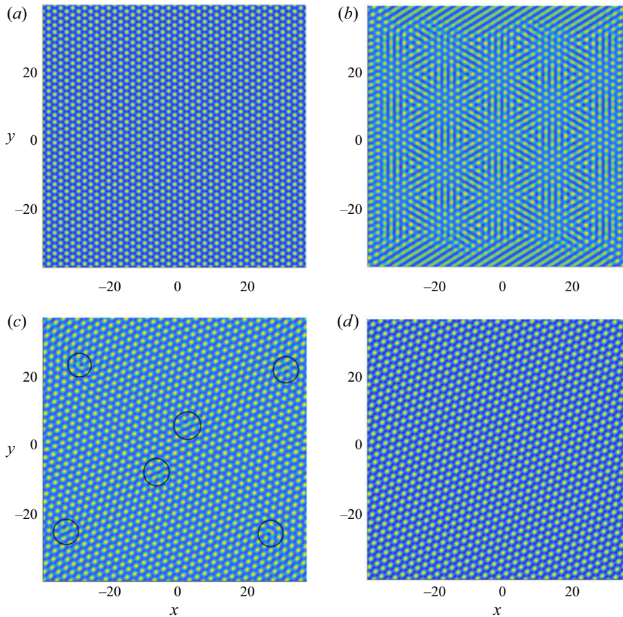
FIGURE 21. Initial condition ( \mathcal{P}_1 ): hexagons with q = 0.45 , \epsilon = 0.1 , r = 2.5 , \alpha = 10^{-4} and Pr = 50 . Contours of the vertical velocity w = \sum_{i=1}^3 A_i \exp(i\mathbf{k}_{c,i} \cdot \mathbf{x}) + \text{c.c.} for a hexagonal pattern undergoing the transverse instability. The contours are shown at times (a) t = 0 ; (b) t = 10 ; (c) t = 1000 and (d) t = 2000 . In panel (c) the penta-hepta defects are circled.
