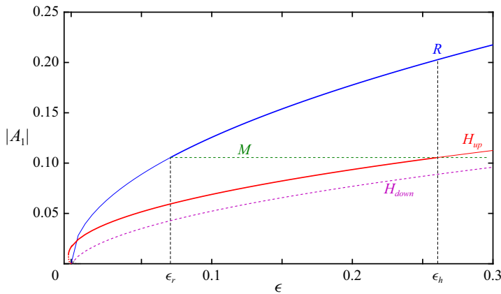
FIGURE 15. Bifurcation diagram for hexagons in the case where g_2 > g_1 with the parameters r = 2.5, q = 0 and \alpha = 10^{-4} . The amplitude |A_1| is plotted against the distance to the threshold \epsilon for the roll-solution branch (labelled R ), for the mixed mode branch (labelled M ) and for the two hexagon-solution branches, up- and down-hexagons. Solid lines indicate stable solutions and dashed lines represent unstable solutions.
