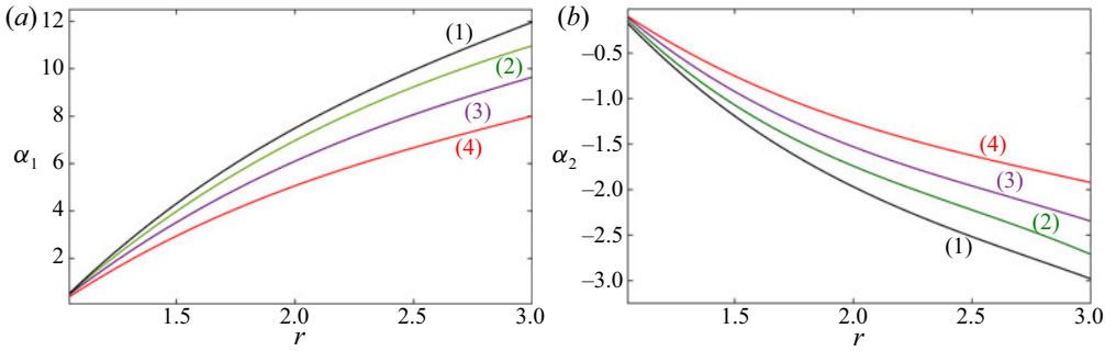
FIGURE 11. Coefficients \alpha_1 and \alpha_2 as a function of r for different values of Pr . (1) Pr = 50 ; (2) Pr = 5 ; (3) Pr = 2 ; (4) Pr = 1 .
