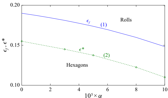
FIGURE 26. Threshold for hexagon–roll transition in the case where there is no distortion of hexagons as a function of the shear-thinning degree, with q = 0.55 , r = 2.5 and Pr = 50 . (1) Curve of equal energy for hexagons and rolls, (2) numerical simulations.
