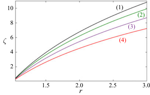
FIGURE 9. Variation of \zeta with the ratio viscosity r for different values of the Prandtl number. (1) Pr = 50 ; (2) Pr = 5 ; (3) Pr = 2 ; (4) Pr = 1 .
