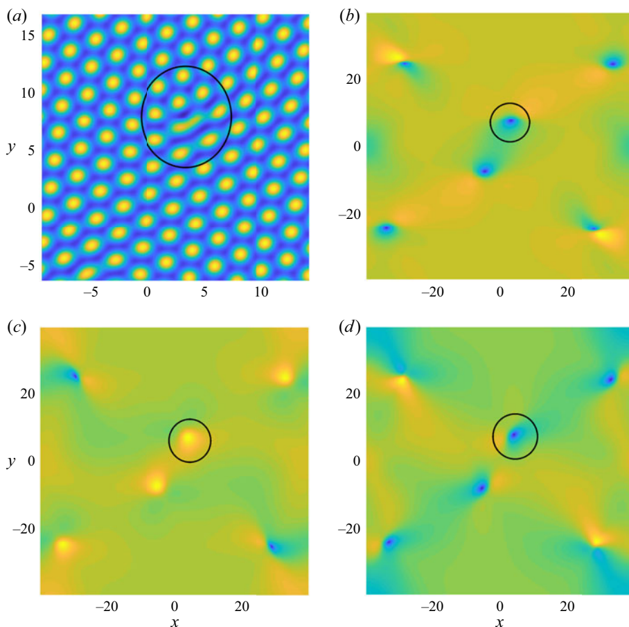
FIGURE 22. Initial condition ( \mathcal{P}_1 ): hexagons with q = 0.45 , \epsilon = 0.1 , r = 2.5 , \alpha = 10^{-4} and Pr = 50 . Focus on one penta-hepta defect at q = 0.45 , r = 2.5 and \alpha = 10^{-4} : (a) contours of the ‘vertical velocity’ w at t = 1000 with one penta-hepta defect circled. (b) Modulus of A_1 which vanishes at the core of the defect. (c) Modulus of A_2 , non-zero in the circle ( |A_2| = 0.114 ). (d) Modulus of A_3 which vanishes at the core of the defect.
