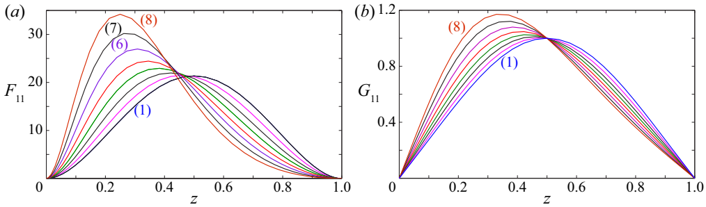
FIGURE 2. Exponential fluid. (a) Vertical velocity eigenfunction and (b) temperature perturbation at the first order as a function of the depth z for different values of the thermodependency coefficient c . (1) c = 0 ; (2) c = 1 ; (3) c = 2 ; (4) c = 3 \dots increasing c by step 1 until curve (8) c = 7 .
