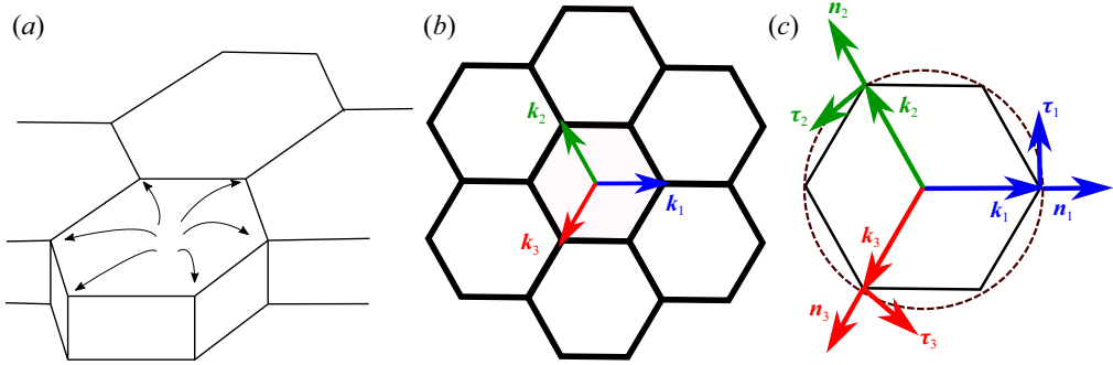
FIGURE 3. (a) Hexagonal convection with flow up in the centre. (b) Basic wavevectors of hexagonal pattern. (c) Unit vectors: n_i parallel and \tau_i perpendicular to the wavevector.
