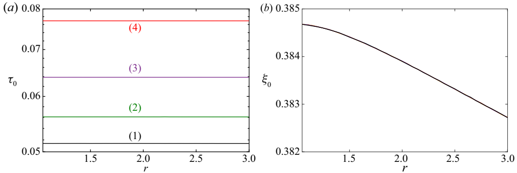
FIGURE 8. Variation of the characteristic time \tau_0 (a) and the coherence length \xi_0 (b) as a function of the viscosities ratio, for different values of Prandtl number. (1) Pr = 50 ; (2) Pr = 5 ; (3) Pr = 2 ; (4) Pr = 1 .
