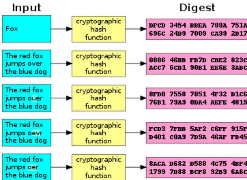
Figure 2. A cryptographic hash function (i.e. SHA-1) at work (Wikipedia, n.d.-a).
