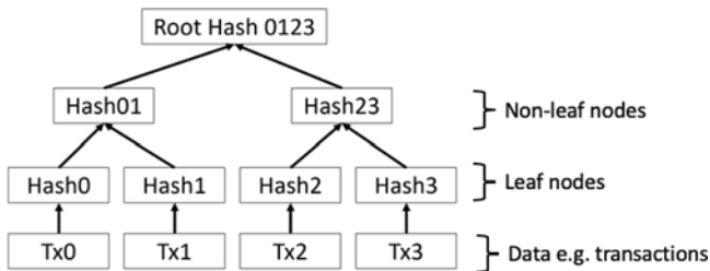
Figure 4. Transactions hashed in a Merkle Tree (Nakamoto, 2008).
