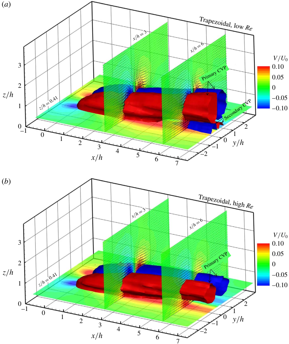
FIGURE 11. (Colour online) The counter-rotating vortex pair in the wake of the trapezoidal tab illustrated with x -vorticity isosurfaces \omega_x h/U_0 = +0.1 (red) and -0.1 (blue) at the low (a) and high (b) Re_h . The V/U_0 contours and in-plane velocity vector fields in y - z planes at x/h=3 and 6 and in the x - y plane at z/h=0.41 are superimposed for clarity. The results are obtained from the volumetric PIV measurements.
