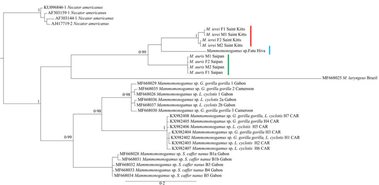
Fig. 5. Phylogenetic tree resulting from Bayesian inference of 420 bp of cox1 gene sequences of Mammomonogamus spp. originating from domestic cats ( M. ierei , M. auris , Mammomonogamus sp. from Fatu Hiva), water buffalo ( M. laryngeus ) and African herbivores. Based on the topology of the tree resulting from the analysis of nuclear DNA, Necator americanus was used as an outgroup. Node-supporting values refer to BI posterior probability (values above 0.9 displayed only). Red line marks the samples from Saint Kitts, blue line the samples from Fatu Hiva and green line is for the samples from Saipan. F, female; M, male; CAR, Central African Republic.
